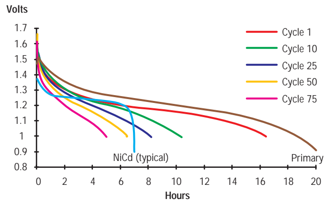
Graph 1: Discharge Profile Comparison Primary Alkaline, NiCd, and Rechargeable Alkaline—100mA Discharge to 1.0V
