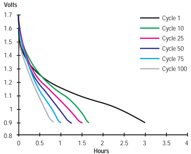
Graph 7: AA Cell Cycle Capacities—300 mA Discharge
