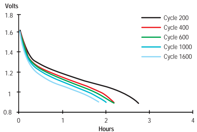
Graph 11: Reserve Capacity After Repeated Short Cycles (Full discharge at 300 mA after every 200th shallow discharge)
