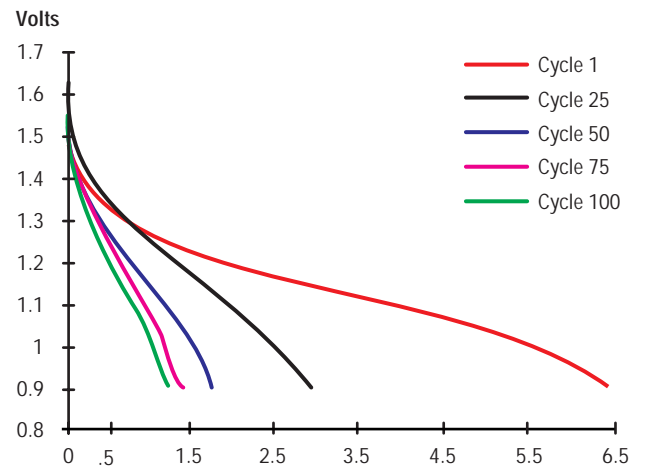
Graph 25: AAA Cell Cycle Capacities—100 mA
