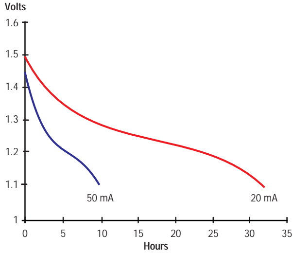
Graph 22: AAA Cell Initial Capacity—Low Current Discharge
