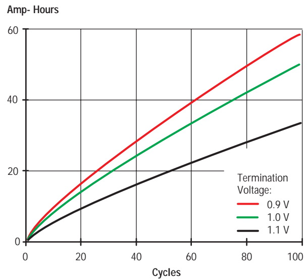
Graph 32: AA Cell Life-Cycle Capacity—200 mA Load
