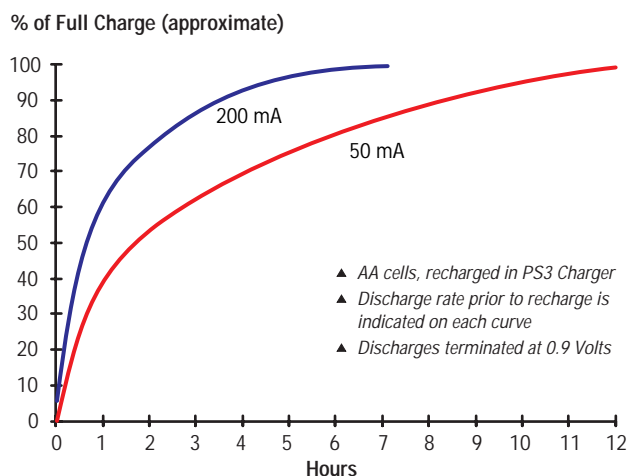
Graph 29: Charge Time for Different Discharge Conditions
