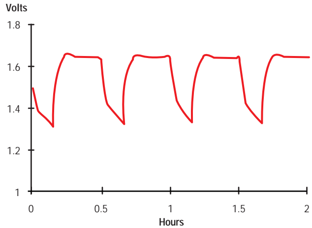
Graph 10: AA Cell Repetitive Short Discharge—Cycles 1797-1800 (400 mA for 10 minutes, recharge after each discharge)
