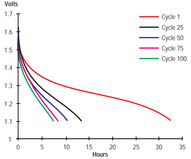
Graph 24: AAA Cell Cycle Capacities—20mA
