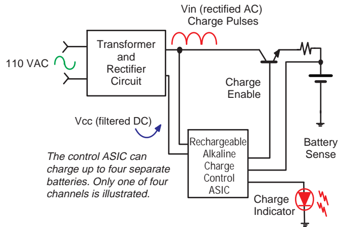
Graph 28: Rechargeable Alkaline Charger Block Diagram
