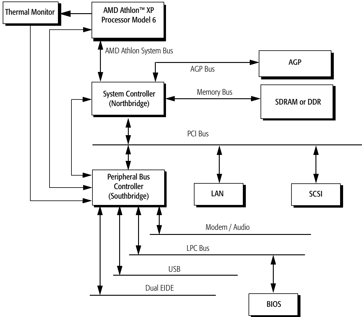
Figure 1. Typical AMD Athlon™ XP Processor Model 6 System Block Diagram
