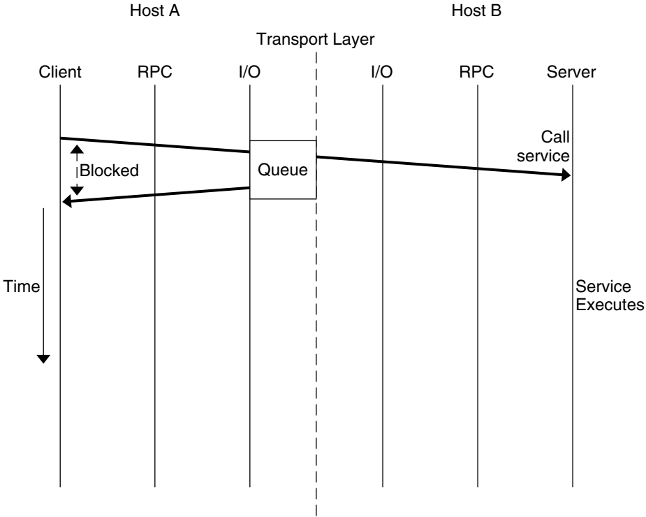
FIGURE 8-1 One-Way Messaging
