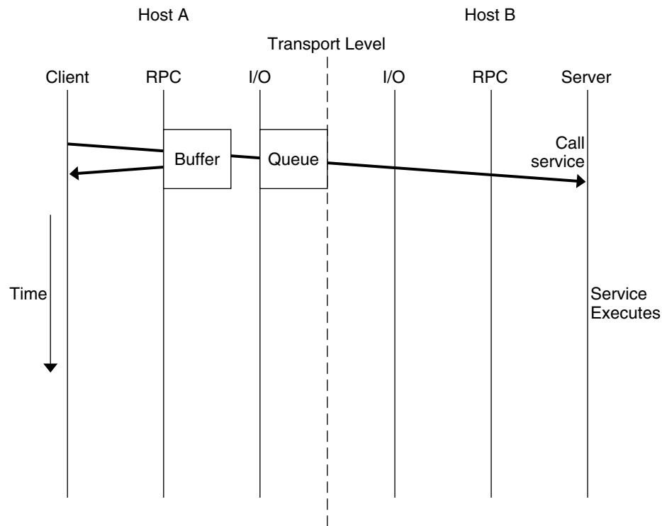
FIGURE 8-3 Non-Blocking Messaging
