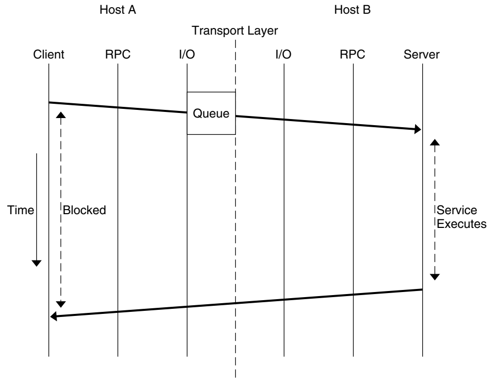
FIGURE 8-2 Two-Way Messaging
