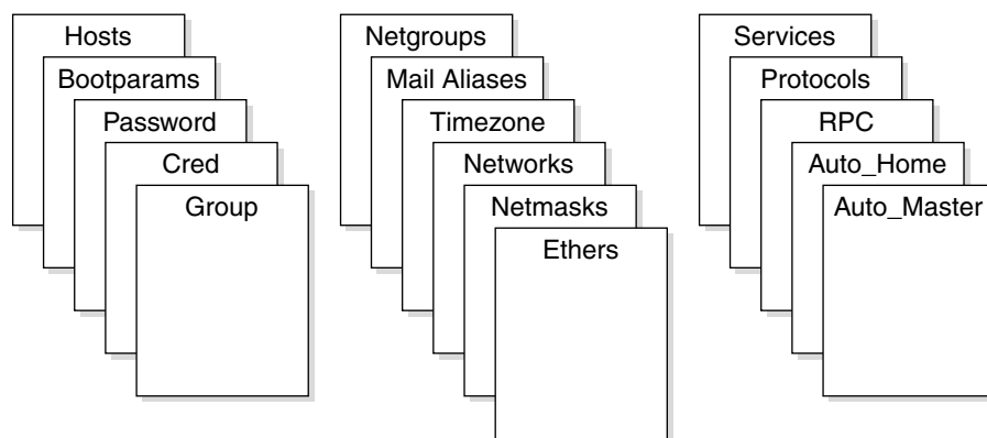
FIGURE 9-2 NIS+ Tables
