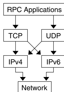
FIGURE 6-1 RPC Applications
