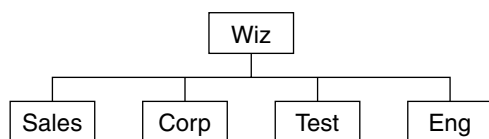
FIGURE 9-1 NIS+ Domain
