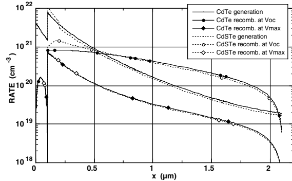
Fig. 9. Generation and recombination rates for devices with and without a CdSTe layer at V_{max} and V_{oc} .
