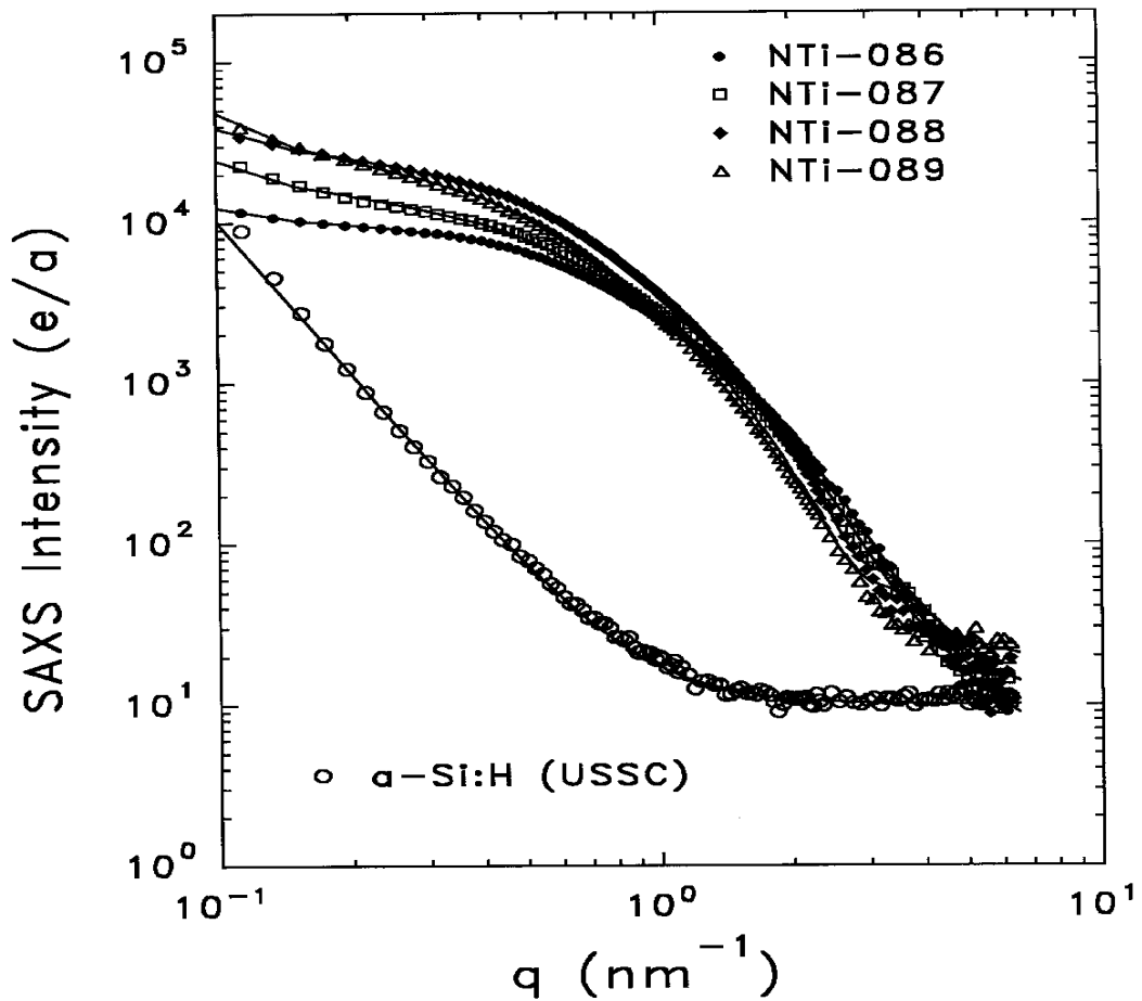
Fig.22. SAXS data from microcrystalline Si:H prepared at the HMI by microwave-PECVD under different substrate biases. PECVD a-Si:H made at USSC shown for comparison.
