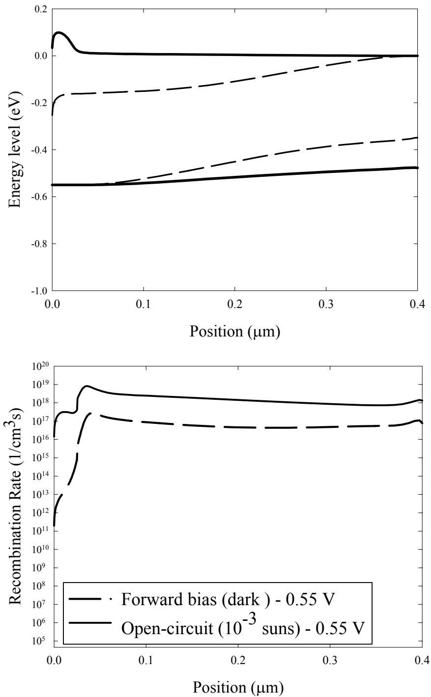
Fig. 23 (a) Simulation of electron and hole quasi-Fermi levels for an a-Si:H p-i-n solar cell obtained under 10^{-3} sun and open-circuit conditions (0.55 V) as well as in the dark under forward bias conditions (0.55 V). (b) Recombination profiles obtained under the same two sets of conditions. In both cases, D^0=10^{18} \text{ cm}^{-3} .
