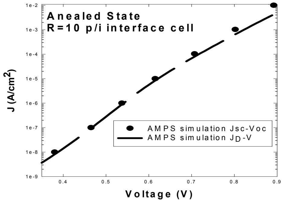
Fig. 21 (a) Dark J-V characteristics of an a-Si:H p-i-n solar cell having an i-layer prepared with R=10 to a thickness of 4000Å (solid line). Also shown are the J_{sc}-V_{oc} pairs for the same solar cell obtained over a wide range of illumination intensity (symbols). (b) AMPS simulation of the superposition of dark J-V and light J_{sc}-V_{oc} characteristics for an R=10 p-i-n solar cell.
