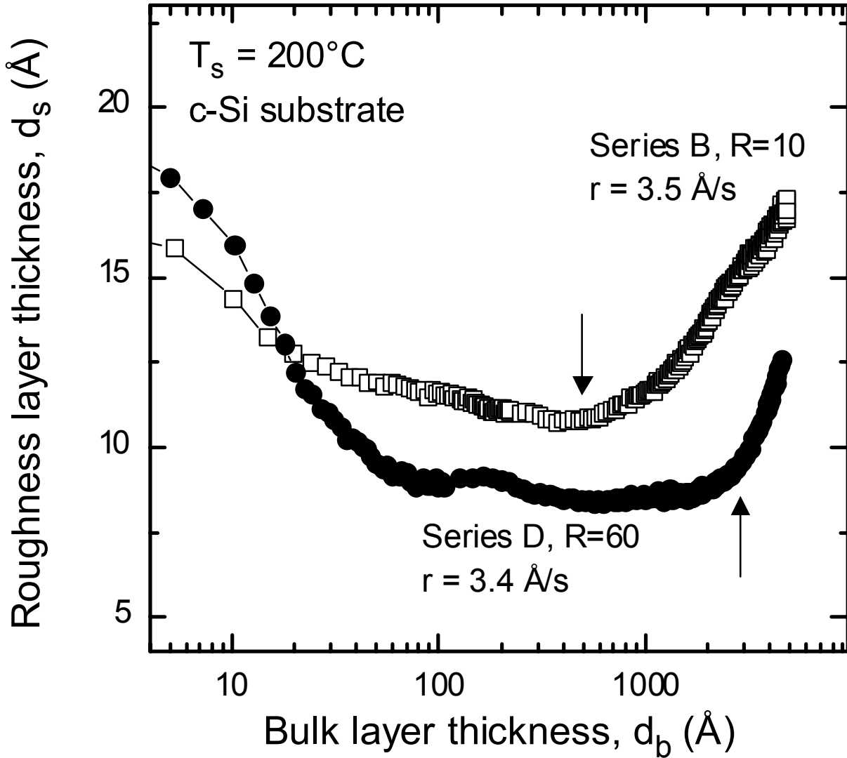
Fig. 10 Surface roughness layer thickness d_s vs. bulk layer thickness d_b for Si:H films prepared on native-oxide-covered c-Si from series B (open squares) and D (filled circles) with different total gas pressures of p_{\text{tot}}=0.4 and 4 Torr, respectively. For the p_{\text{tot}}=0.4 Torr deposition of series B , the rf plasma power was 0.8 \text{ W/cm}^2 and the \text{H}_2 dilution ratio was R=10 , yielding a rate of 3.5 \text{ \AA/s} . For the p_{\text{tot}}=4 Torr deposition of series D , the power was 0.3 \text{ W/cm}^2 and the \text{H}_2 dilution ratio was R=60 , yielding a similar rate of 3.4 \text{ \AA/s} . For the film with p_{\text{tot}}=0.4 Torr, the a \rightarrow a roughening transition occurs near d_b=500 \text{ \AA} , whereas for the film with p_{\text{tot}}=4 Torr, the a \rightarrow (a+\mu\text{c}) roughening transition occurs near d_b=3000 \text{ \AA} .
