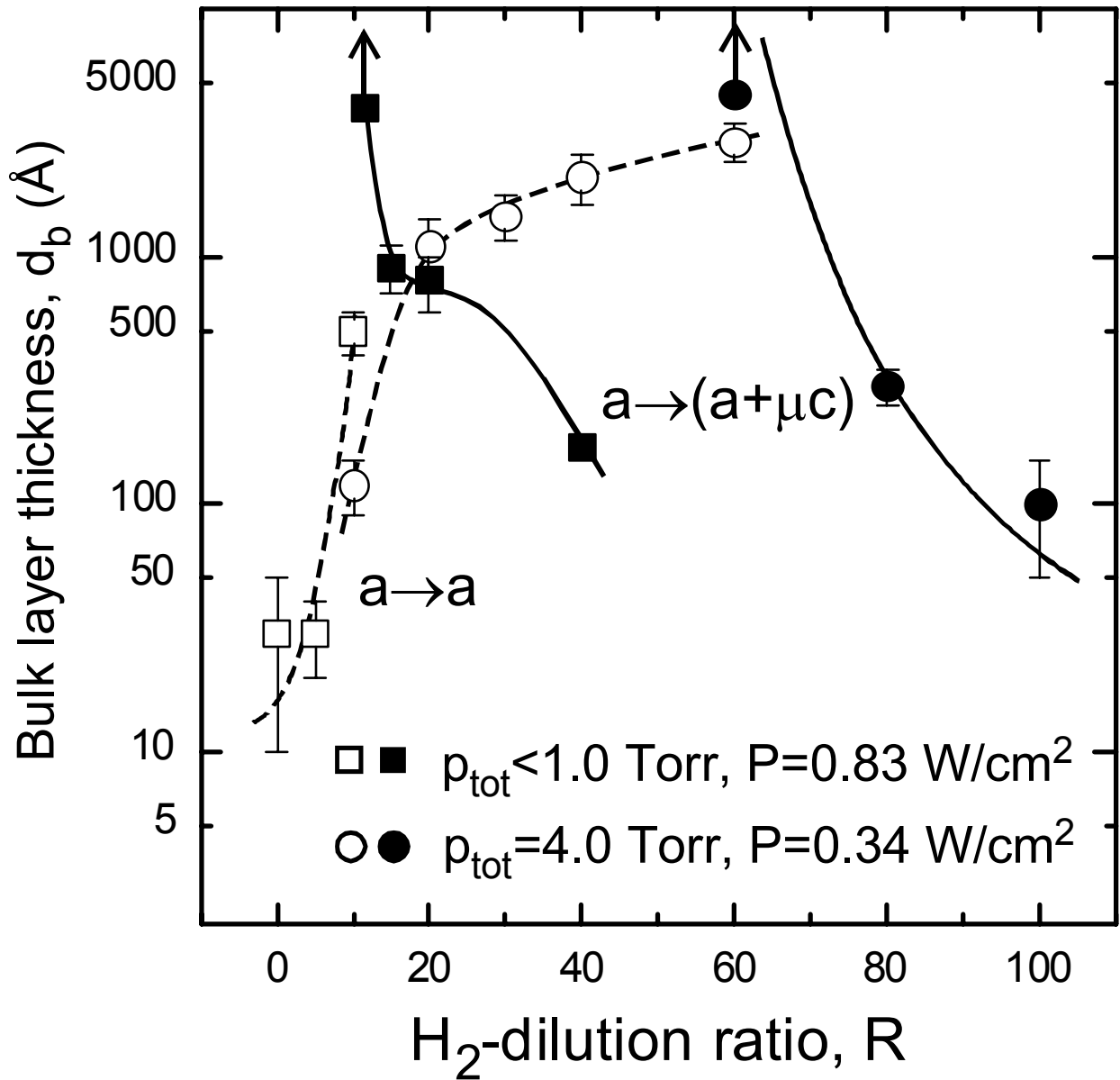
Fig. 11 Comparison between the phase diagrams for Si:H film deposition on c-Si for series B (squares) and series D (circles). The deposition parameters are P=0.8 W/cm 2 and p_{tot}<1 Torr for series B , and P=0.3 W/cm 2 and p_{tot}=4.0 Torr for series D . The open symbols and broken lines indicate the amorphous-to-amorphous roughening transitions [ a \rightarrow a ], and the filled symbols and solid lines indicate the amorphous-to-(mixed-phase-microcrystalline) transitions [ a \rightarrow (a + \mu c) ]. The up arrows indicate that the transition occurs above the indicated thicknesses.
