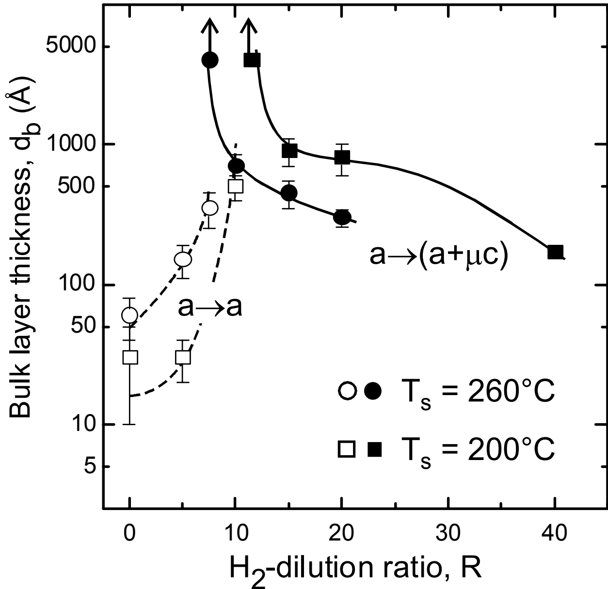
Fig. 9 Comparison between the phase diagrams for Si:H film deposition on c-Si at P=0.8 \text{ W/cm}^2 and two different substrate temperatures: T=200^\circ\text{C} (series B - squares) and 260^\circ\text{C} (series C - circles). The open symbols and broken lines indicate the amorphous-to-amorphous roughening transitions [ a \rightarrow a ], and the filled symbols and solid lines indicate the amorphous-to-(mixed-phase-microcrystalline) transitions [ a \rightarrow (a+\mu c) ]. The up arrows indicate that the transition occurs above the indicated thicknesses.
