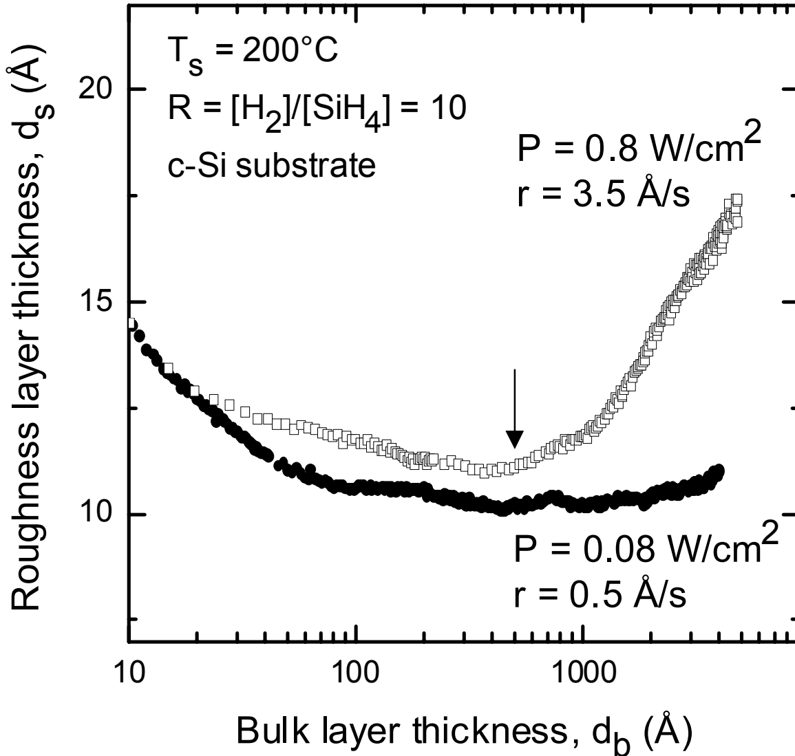
Fig. 4 Surface roughness layer thickness d_s as a function of bulk layer thickness d_b for a-Si:H films prepared on native-oxide-covered c-Si with fixed T=200^\circ\text{C} and R=10 , but different rf power levels of P=0.08 \text{ W/cm}^2 (series A – filled circles) and 0.8 \text{ W/cm}^2 (series B – open squares). For the higher P film, an amorphous-to-amorphous surface roughening transition (a→a) occurs near d_b=500 \text{ \AA} (arrow), whereas for the lower P film, any such transition must occur for d_b>4000 \text{ \AA} .
