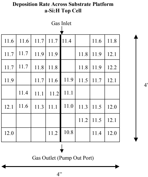
Figure 12. Deposition rate distribution across the substrate platform at low pressure conditions.
