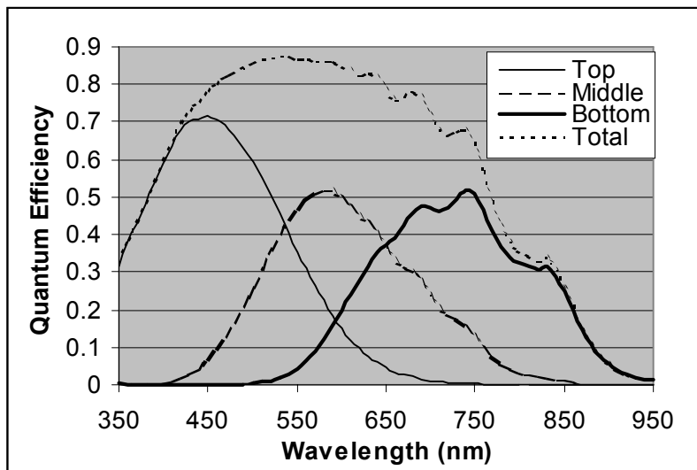
Figure 16. Quantum efficiency plot for triple-junction cell made using VHF technique. Top Cell Current =6.9 mA/cm 2 , Middle Cell Current =7.1 mA/cm 2 , Bottom Cell Current =7.8 mA/cm 2 .
