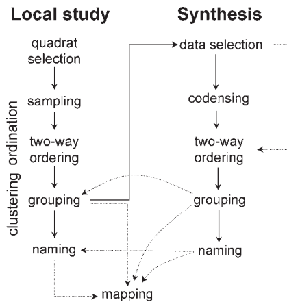
Fig. 1. Structure of Central European phytosociological research and its analogy to multivariate statistics; dashed lines show optional pathways including the feedback from synthetic to subsequent local work.
