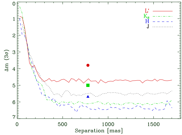
Fig. 2. Detection limits at 3\sigma achieved during our observations in J-band (dotted black line), H-band (dashed blue line), K_s -band (dashed-dotted green line) and L' -band (solid red line). The contrasts between 2M1207 and its GPCC are reported for H (filled triangle), K_s (filled box) and L' (filled circle) (the GPCC was not detected in J band).
