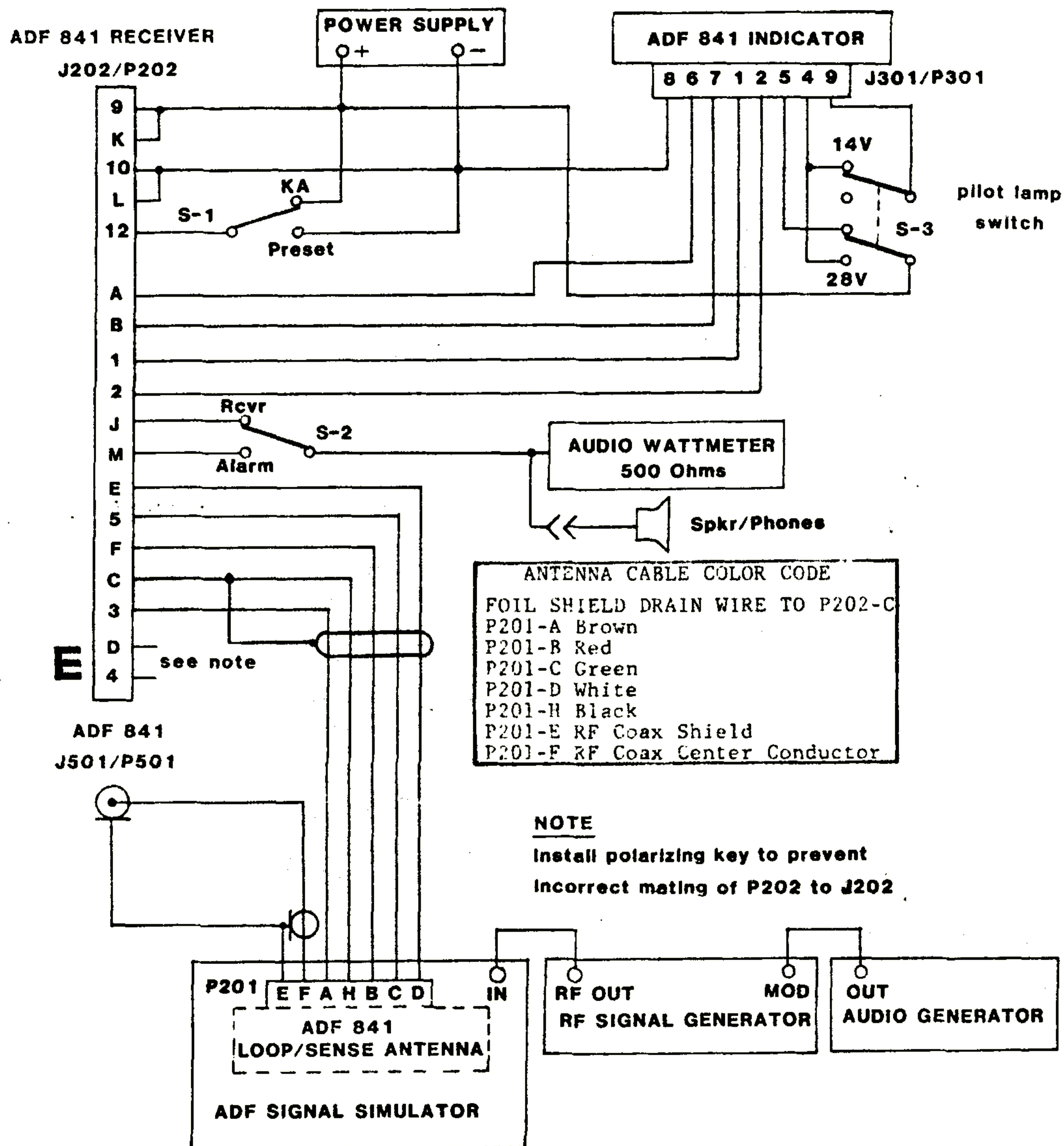
FIGURE 2-1 BENCH TEST SET-UP AND CABLE WIRING
