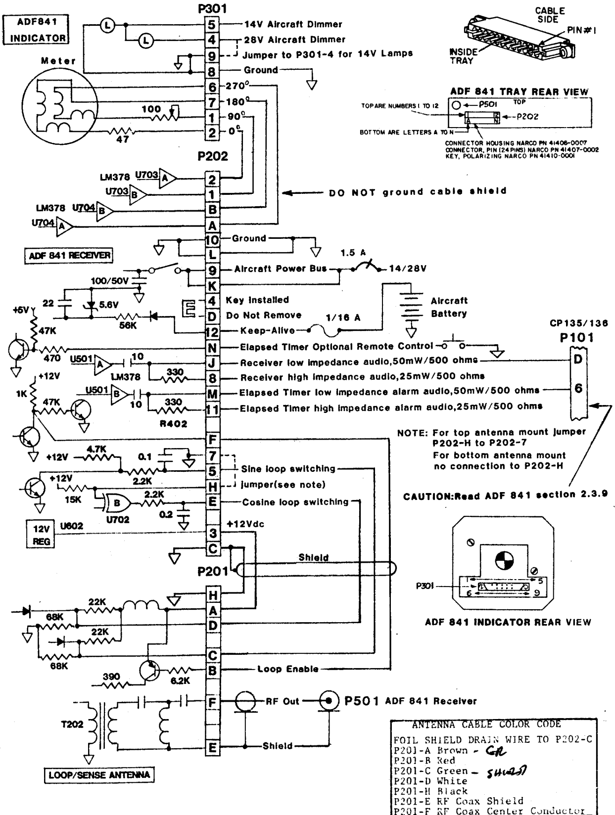
FIGURE 2-3 ADF-841 TSO SYSTEM INTERCONNECT WIRING DIAGRAM
