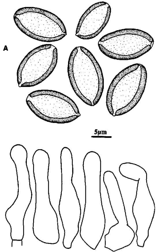
Fig. 8 Psilocybe subcoprophila (PDD 57479): A, spores; B, cheilocystidia.
