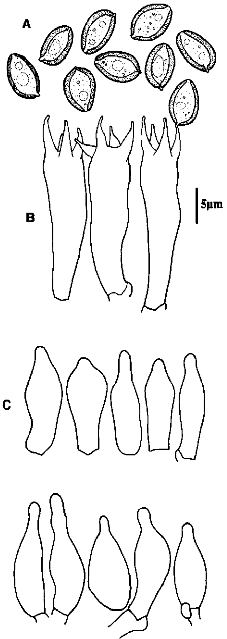
Fig. 4 Psilocybe makarorae (PDD 57396 – holotype): A, spores; B, basidia; C, pleurocystidia; D, cheilocystidia.
