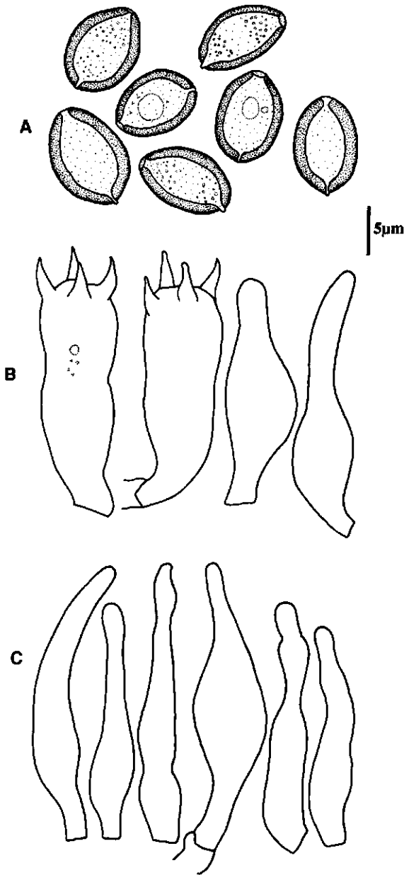
Fig. 3 Psilocybe coprophila (PDD 48412): A, spores; B, basidia; C, cheilocystidia.
