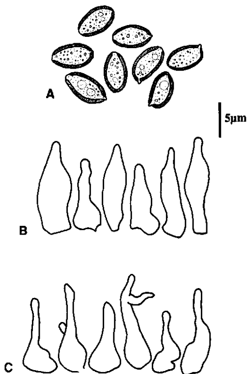
Fig. 2 Psilocybe aucklandii (PDD 58423): A, spores; B, pleurocystidia; C, cheilocystidia.
