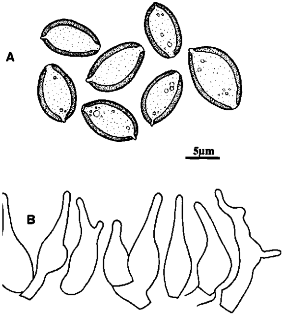
Fig. 6 Psilocybe semilanceata (PDD 46727): A, spores; B, cheilocystidia.
