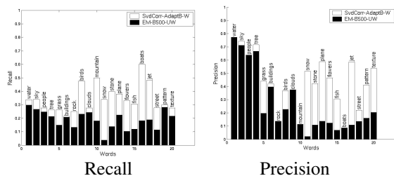
Figure 3. Recall and precision of the top 20 frequent words in the test set. SvdCorr (white bars) gives more general performance than EM (black bars).
