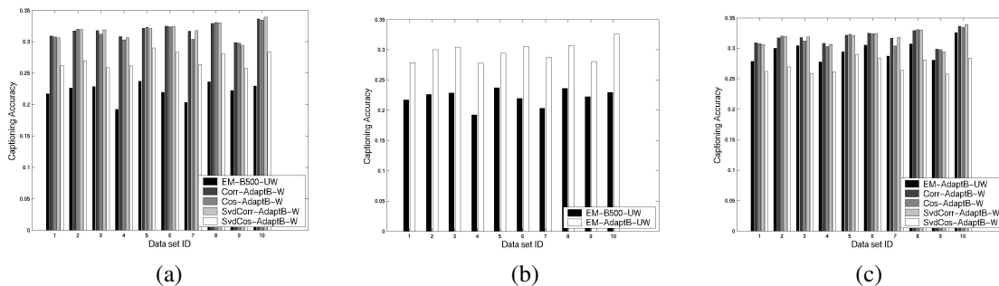
Figure 2. Captioning accuracy improvement (a) proposed methods vs. the baseline EM-B500-UW , (b) adaptive blob-token generation on EM vs. the baseline, (c) proposed methods vs. EM when the adaptively generated blob-tokens are used.
