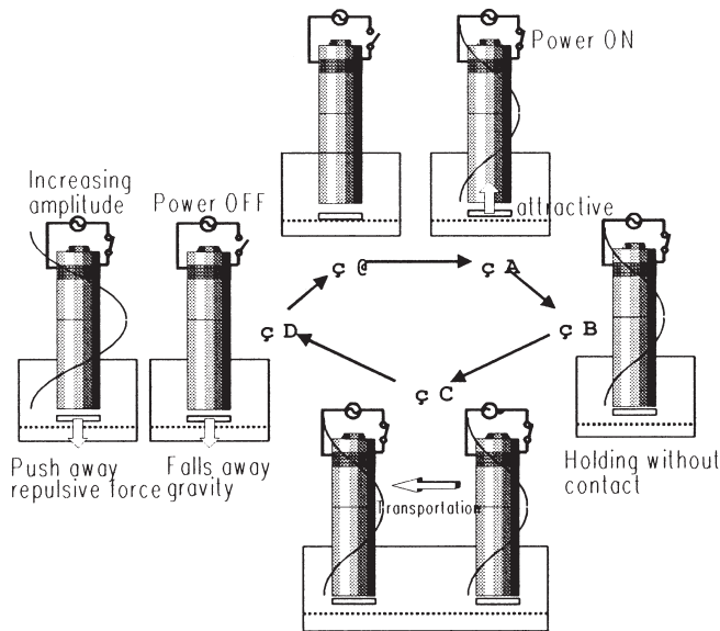
Fig.7. Sequence of non-contact transportation by using an ultrasonic lifter.
