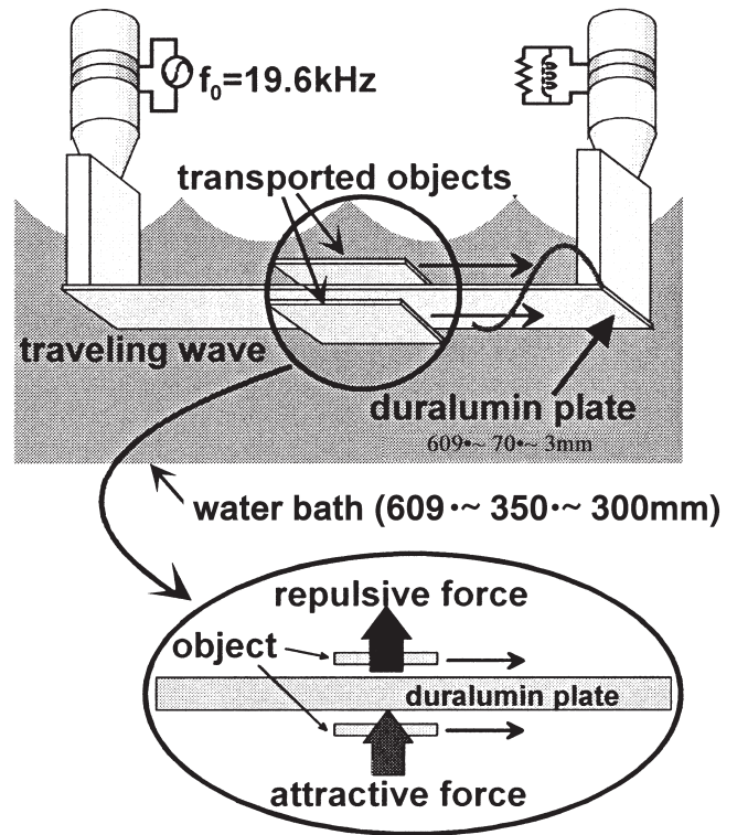
Fig.6. Underwater transportation system using a traveling wave
