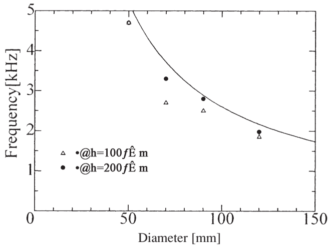
Fig.3. The frequency versus the diameter of the planar object at which attractive force varies to repulsive force. The solid line shows the fundamental resonance frequency of the thin air disk.
