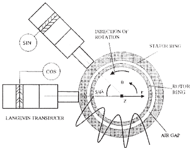
Fig.5. Configuration of ultrasonic motor using NFAL.
