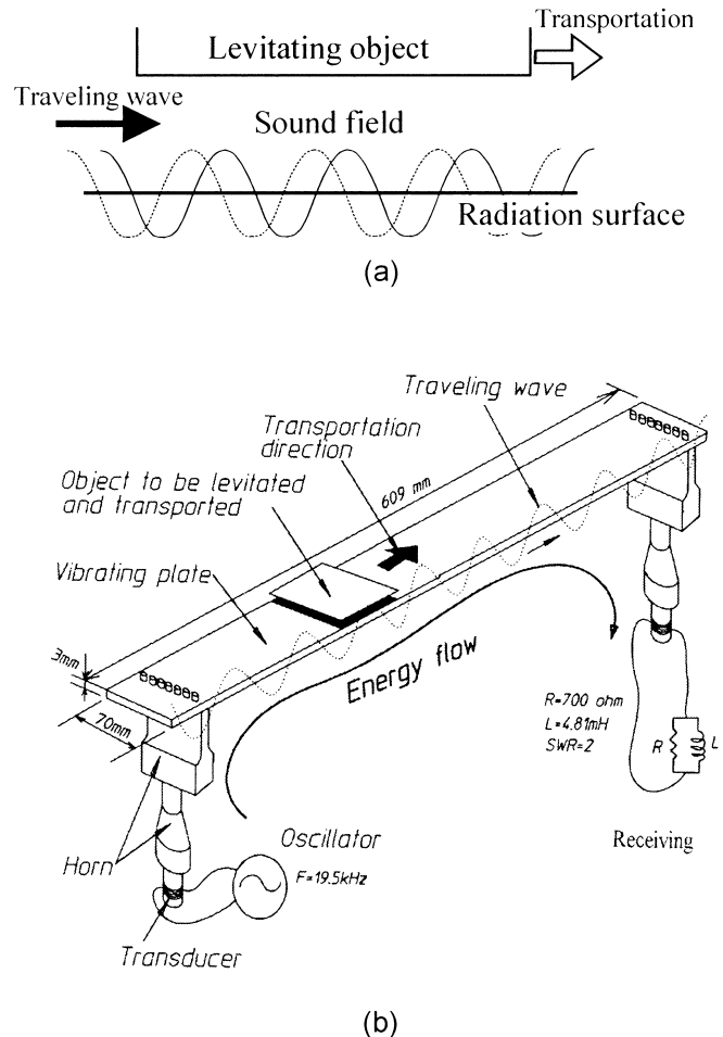
Fig.4. Principle and configuration of transportation system by NFAL. (a) Schematic, (b) Setup configuration.
