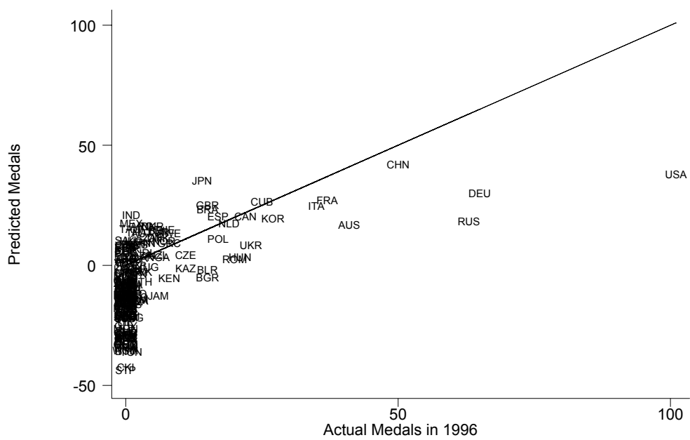
Figure 1: Predicted and actual medal totals for 1996 from the specification in Table 2, column II. (Points on the diagonal line represent perfect predictions.)
