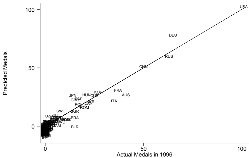
Figure 2: Predicted and actual medal totals for 1996 from the specification in Table 2, column IV. (Points on the diagonal line represent perfect predictions.)
