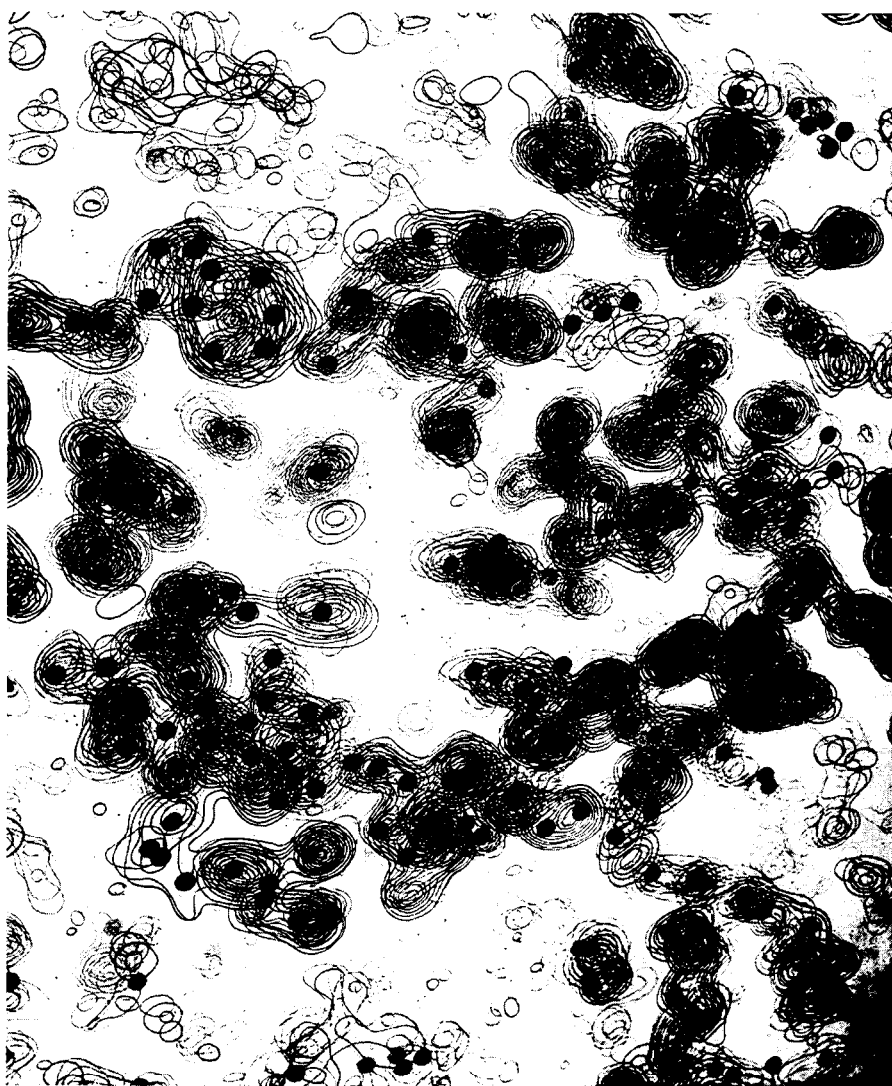
Fig. 11. Part of the 1.4\text{\AA} Fourier synthesis. ( Left centre ) a tryptophan residue; ( to the left ) a liquid region between two molecules.
