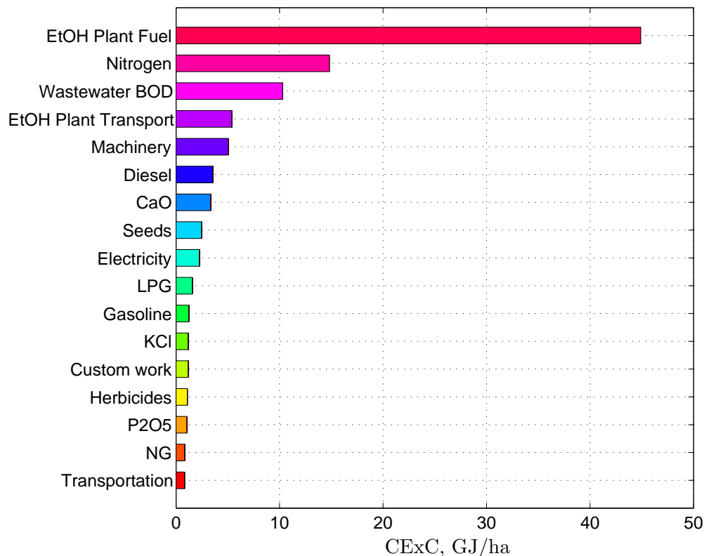
Figure 42: The specific cumulative exergy consumption (CExC) by each major non-renewable resource input to the industrial corn-ethanol cycle.
