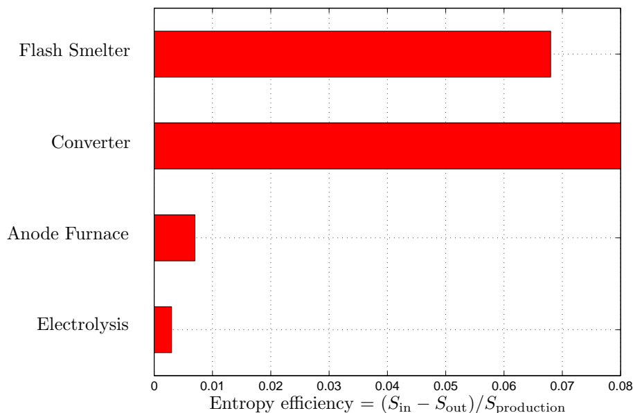
Figure 21: The Second Law efficiency of copper production is incredibly small. The steps in sorting the copper atoms are: Ore Concentration 2% \rightarrow 30% Cu (not shown); Smelter 30% \rightarrow 63% Cu; Converter 63% \rightarrow 99.1% Cu; Anode furnace 99.1% \rightarrow 99.55% Cu; and Electrolysis 99.55% \rightarrow 99.99% Cu. Source: STEFAN GÖSSLING, Entropy Production as a Measure for Resource Use , University of Hamburg, 2001.
