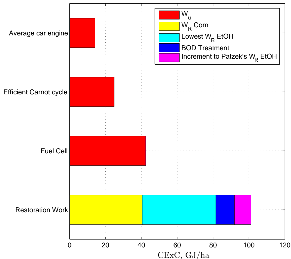
Figure 43: The minimum cumulative exergy consumption by the industrial corn-ethanol cycle and its maximum useful work, W_u . For comparison, the cycle's ethanol is burned in an average car engine, an efficient CARNOT engine, and in an ideal fuel cell. This comparison demonstrates that the industrial corn-ethanol cycle is unsustainable by a factor of 2-7. No adjustment of process parameters I can think of will change this terrible situation. Note that the W_R EtOH bar is the lowest fossil energy use (34 000 Btu/gal+0.75 kWh/gal advertised in 2004 by ICM, 310 North First Street, Colwich, Kansas 67030, www.icmnc.com). The rightmost purple bar shows the difference between the ICM value and my estimate of fossil energy use to produce anhydrous ethanol.
