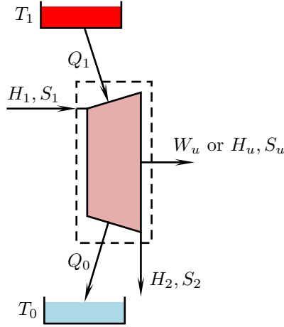
Figure 31: Exergy balance in ideal (reversible) and real (irreversible) nonisothermal industrial process.
