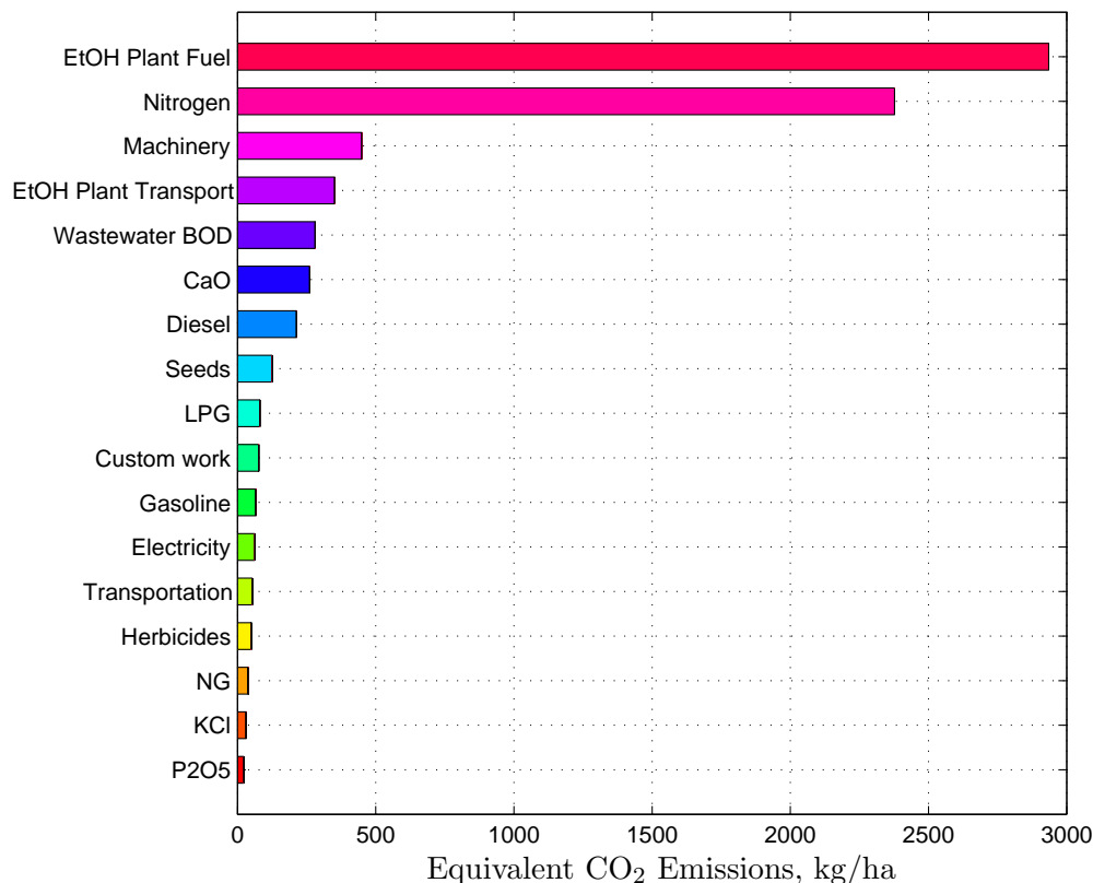
Figure 36: Equivalent CO 2 emissions from each major non-renewable resource consumed by the industrial Corn-EtOH cycle.
