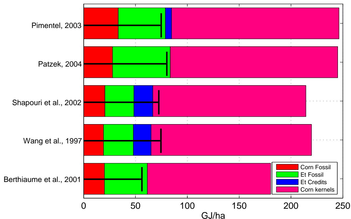
Figure 17: The overall energy balance of ethanol production. The two or three leftmost parts of each bar represent the specific fossil energy used in corn farming and ethanol production. The fossil energy inputs into ethanol production are the sum of the green part and the blue energy credit part for some authors. The rightmost part is the calorific value of corn grain harvested from 1 hectare. The total lengths of the horizontal bars represent all energy inputs into ethanol production. The horizontal lines with the vertical anchors represent the calorific value of ethanol obtained from one hectare of corn. Note that the total energy inputs into ethanol production are equivalent to \sim 4 – 5 metric tonnes of gasoline per hectare. The ethanol's calorific value is equal to 1–1.3 metric tonnes of gasoline.
