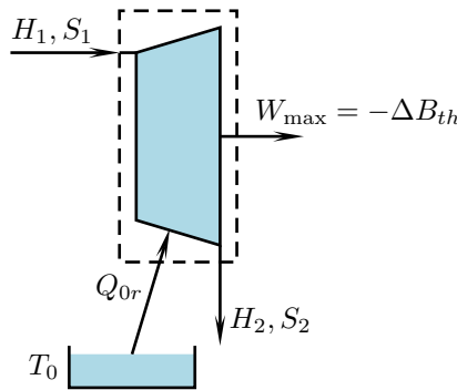
Figure 30: Exergy balance in an isothermal, ideal flow machine. The maximum possible shaft work from this machine is equal to the negative change of thermal exergy.
