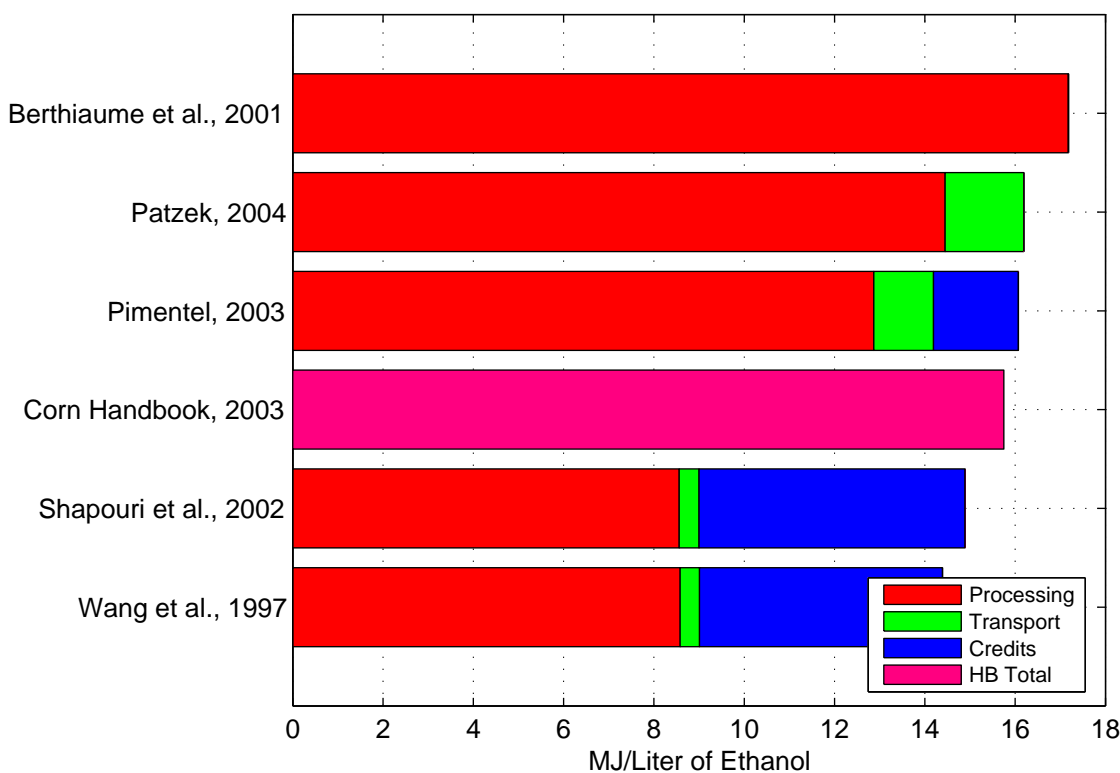
Figure 16: The average fossil energy inputs to ethanol production in a wet milling plant. The length of each bar is the total energy outlay to produce 1 liter of EtOH, and the blue parts denote the size of energy credits assumed by the different authors.
