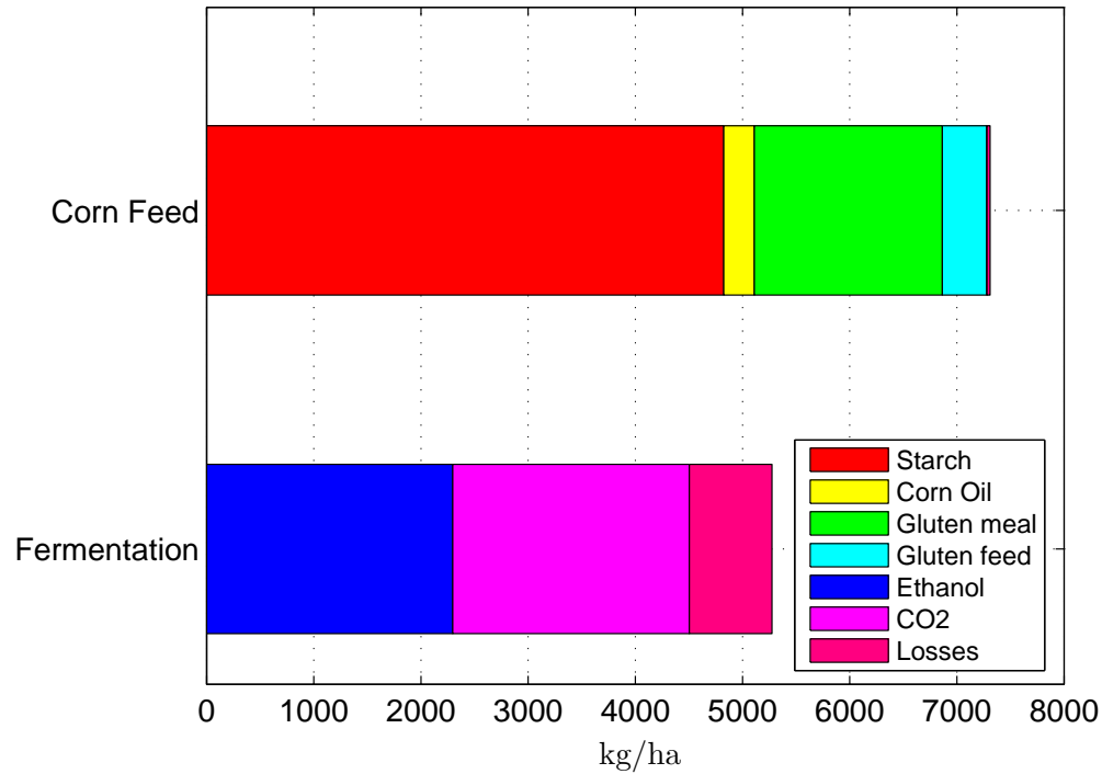
Figure 14: The result of practical corn conversion into ethanol with 16% losses is 0.399 L EtOH/kg dry corn grain = 2.682 gal EtOH/ dry bushel = 2.28 gal EtOH/ wet bushel with 15% moisture. Note that the dry starch is swollen by a factor of 180/162 caused by hydrolysis to glucose.
