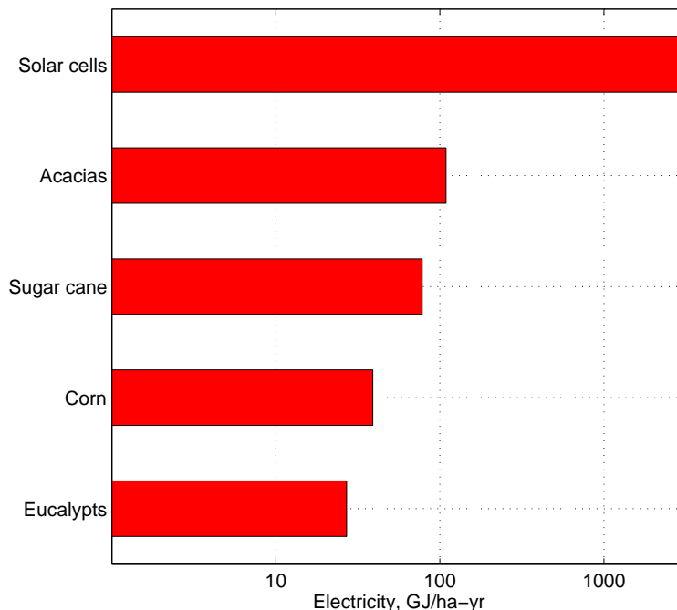
Figure 46: The amount of electricity generated in 1 year with solar cells on 1 ha dwarfs those generated with hydrogen-burning 60%-efficient fuel cells or in power stations. The hydrogen is obtained with no losses from ethanol from corn and sugarcane, and electricity is generated with the 35%-efficiency from eucalypt and acacia wood pellets. The annual electricity yields have been calculated by PATZEK & PIMENTEL (2005). The minimum solar cell yield follows the assumptions in this appendix. Note that the bar scale is logarithmic , and annually the solar cells produce \sim 100 times more electricity than corn ethanol.
