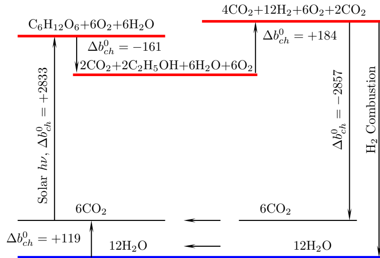
Figure 40: Exergy diagram of the ideal CO 2 -Glucose-EtOH-H 2 cycle.
