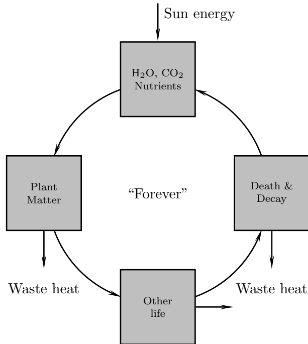
Figure 28: An ecosystem transforms the sun energy (low thermal entropy) into waste heat (high thermal entropy). The waste heat is continuously exported to the universe. Everything else is completely reused, or recycled.
