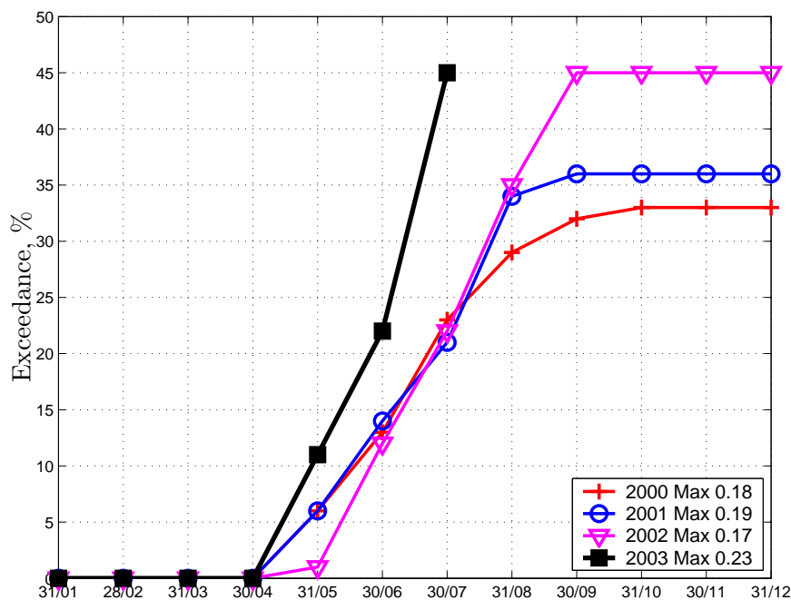
Figure 45: The cumulative one-hour exceedances of maximum legal ozone level in Southern California. Source: CAL HODGE, President of A 2 nd Opinion, Inc.
