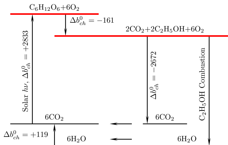
Figure 39: Exergy diagram of the ideal CO 2 -Glucose-EtOH cycle.
