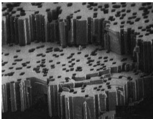
Figure 2: Etched channel profiles and etch pit openings of the etched tracks due to 2380 MeV 84 Kr-ions in the crystalline matrix of a Muscovite mica track detector. The profiles are cylindrical with diamond shaped etch pit openings in the crystalline matrix of mica track detector.
