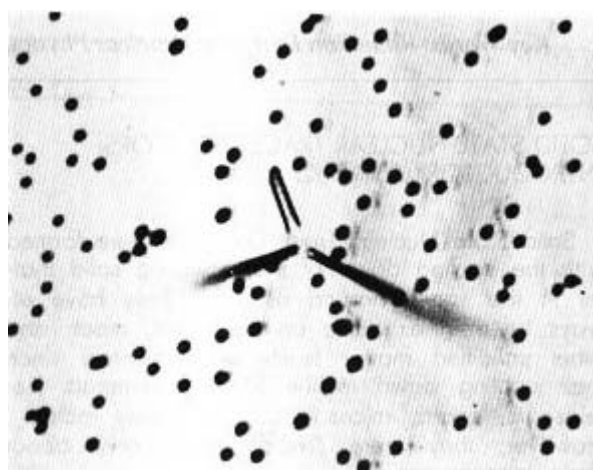
Figure 3: A photomicrograph showing the top view of the etch pits due to energetic 136 Xe-ions in a plastic track detector. A three prong event resulted in the interaction of 136 Xe-ions with a gold target is also present in the photograph.
