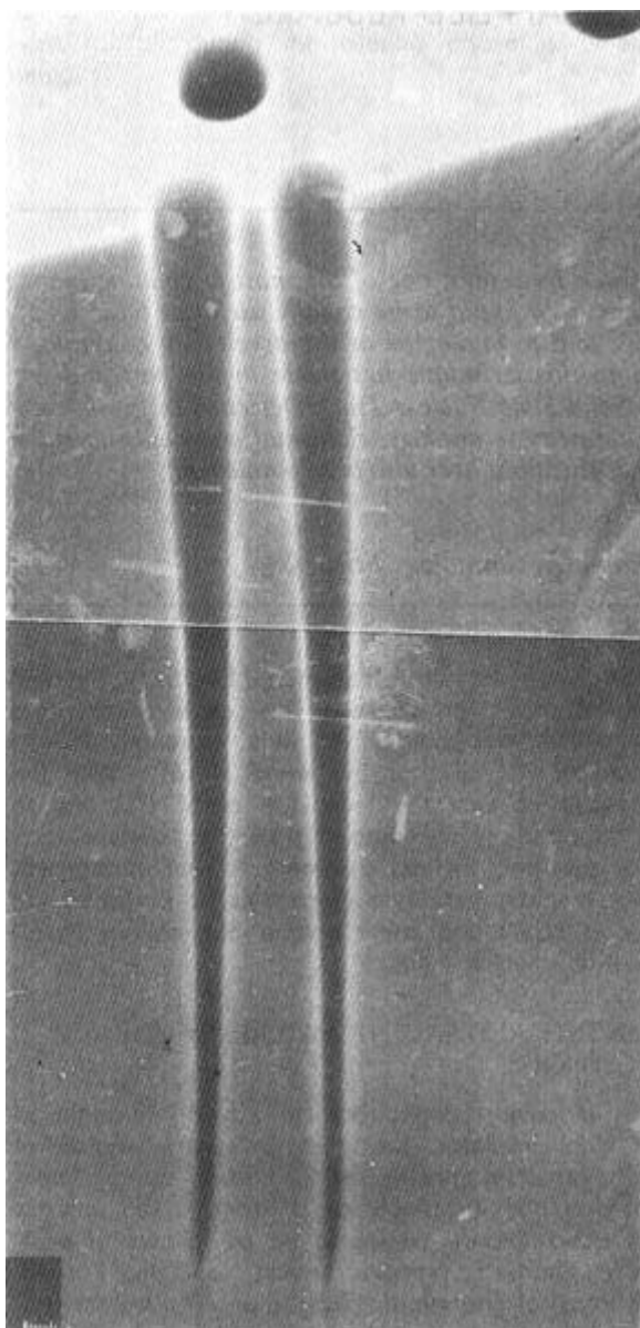
Figure 1: A photomicrograph showing profiles of two long etched tracks along with two etch pits due to energetic uranium ions in a CR-39 (a polycarbonate) plastic track detector. The etched channels are conical in shape and the etch pit openings are uniform in the amorphous matrix of the detector.
