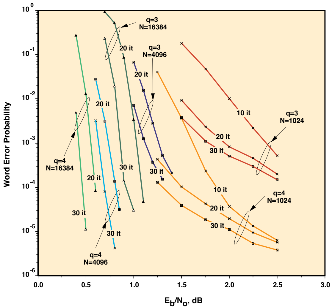
Figure 5. Simulated performance of iterative decoding of RA codes on an AWGN channel.
