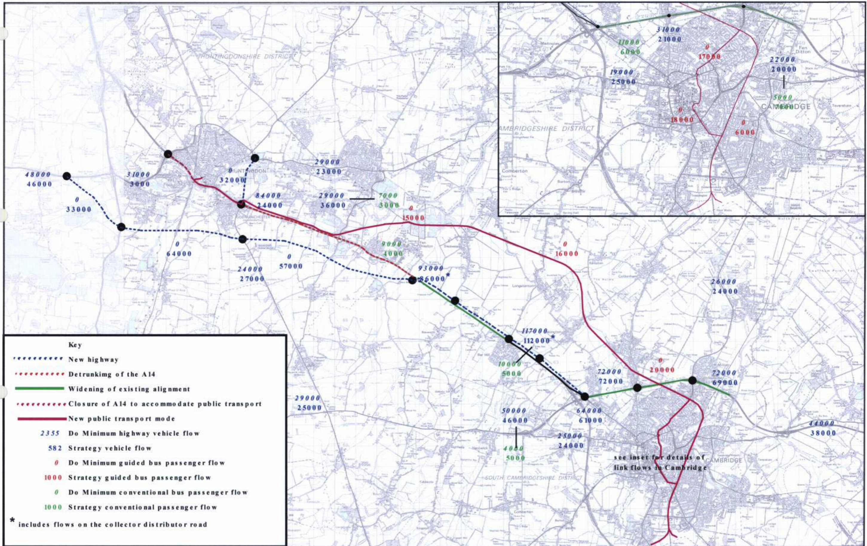
Figure 4.2H Highway and Public Transport Two-Way Daily Flows 2016 Do Minimum and Strategy 2
