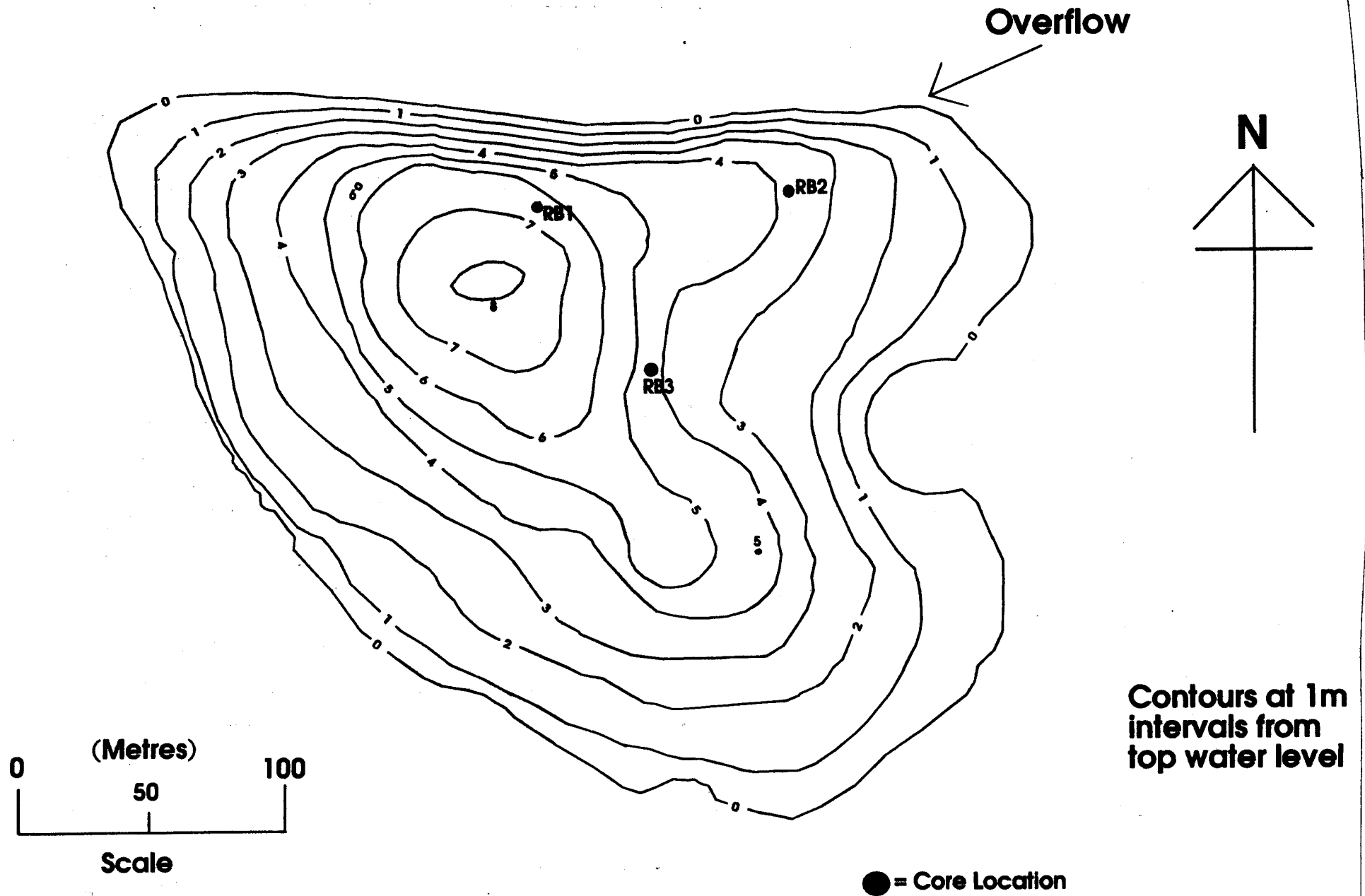
Figure A3.1 Plan of Reservoir C showing Results of Bathymetric Survey and Position of Sediment Sampling Cores
