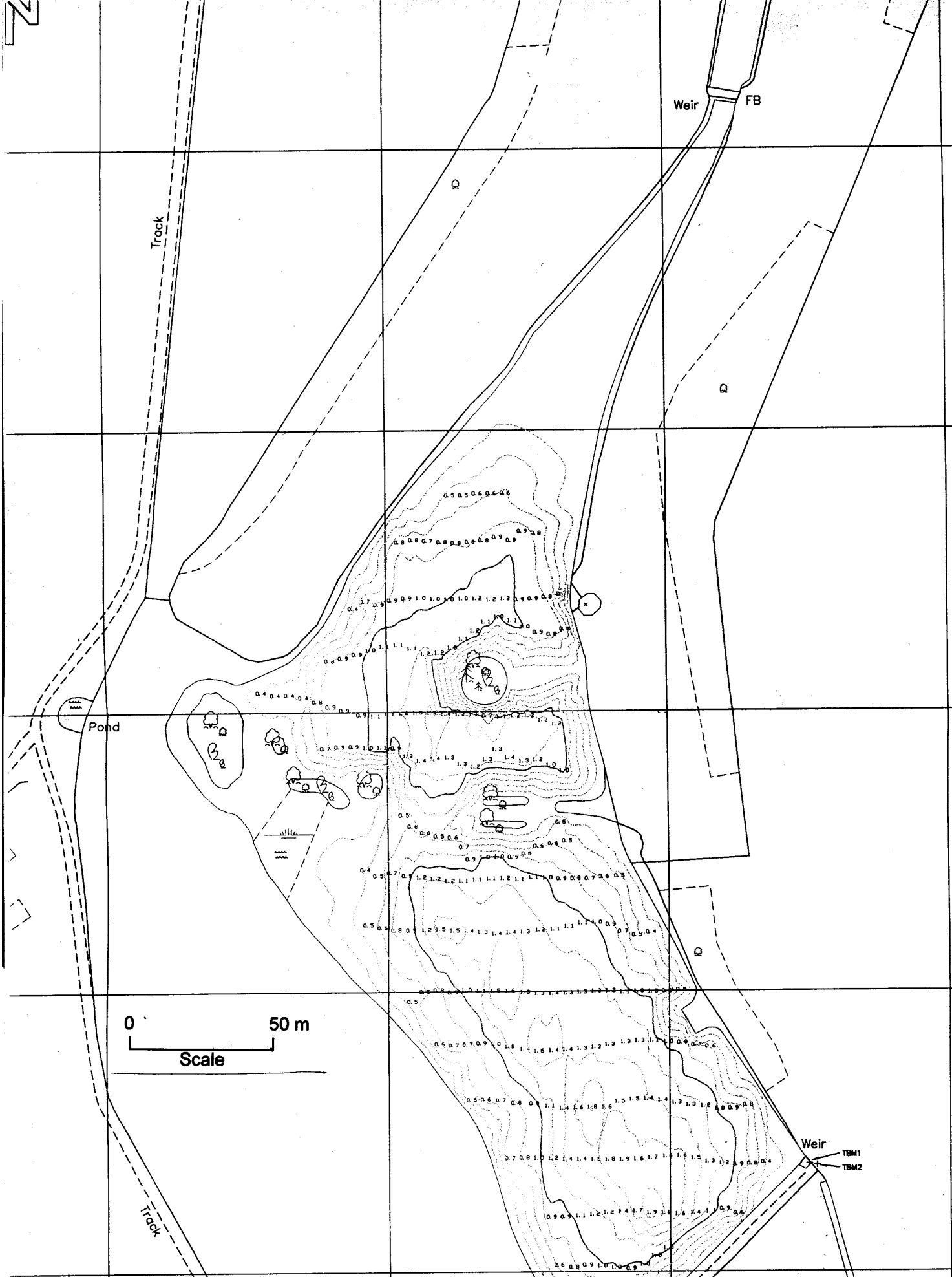
Figure A1.1a Plan of Reservoir A showing Depth to Top of Sediment below Water Level
