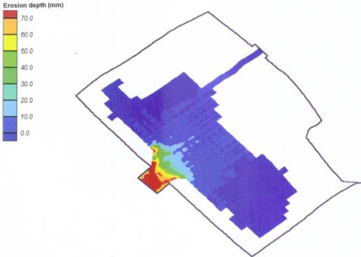
Figure 6.15 Reservoir B Dambreak – Total erosion depth with 'Sunny Day' Inflow Conditions
