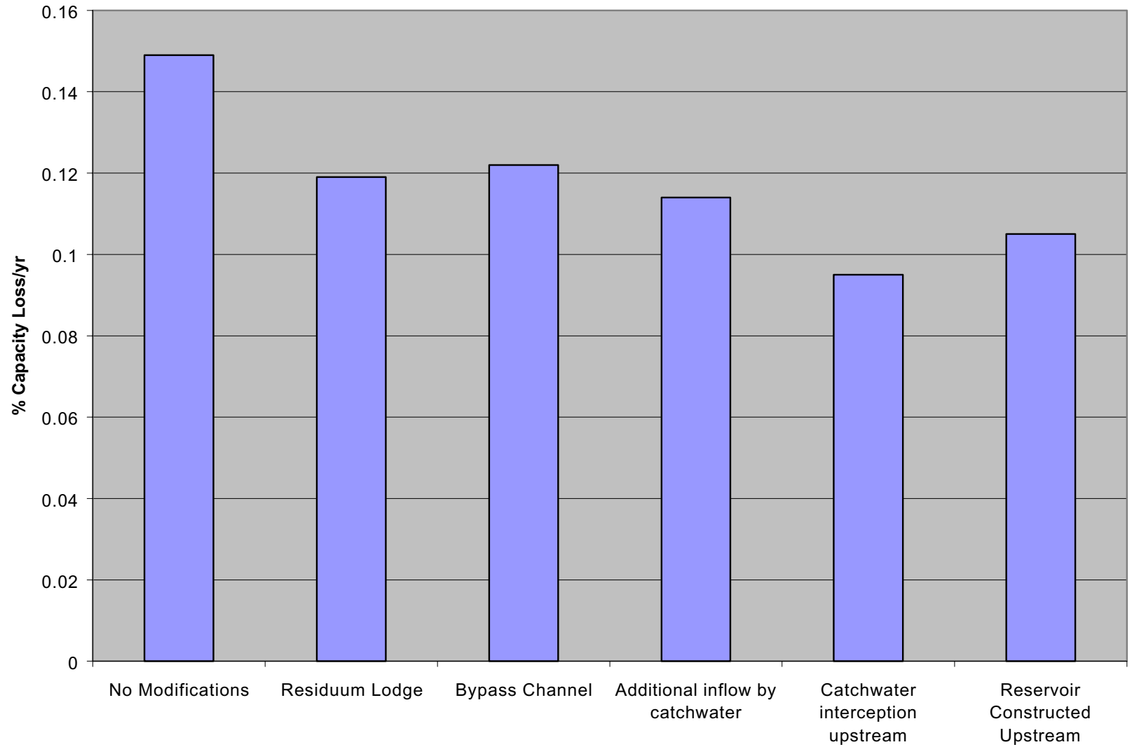
Measurements of long term siltation rates with different sediment control methods
