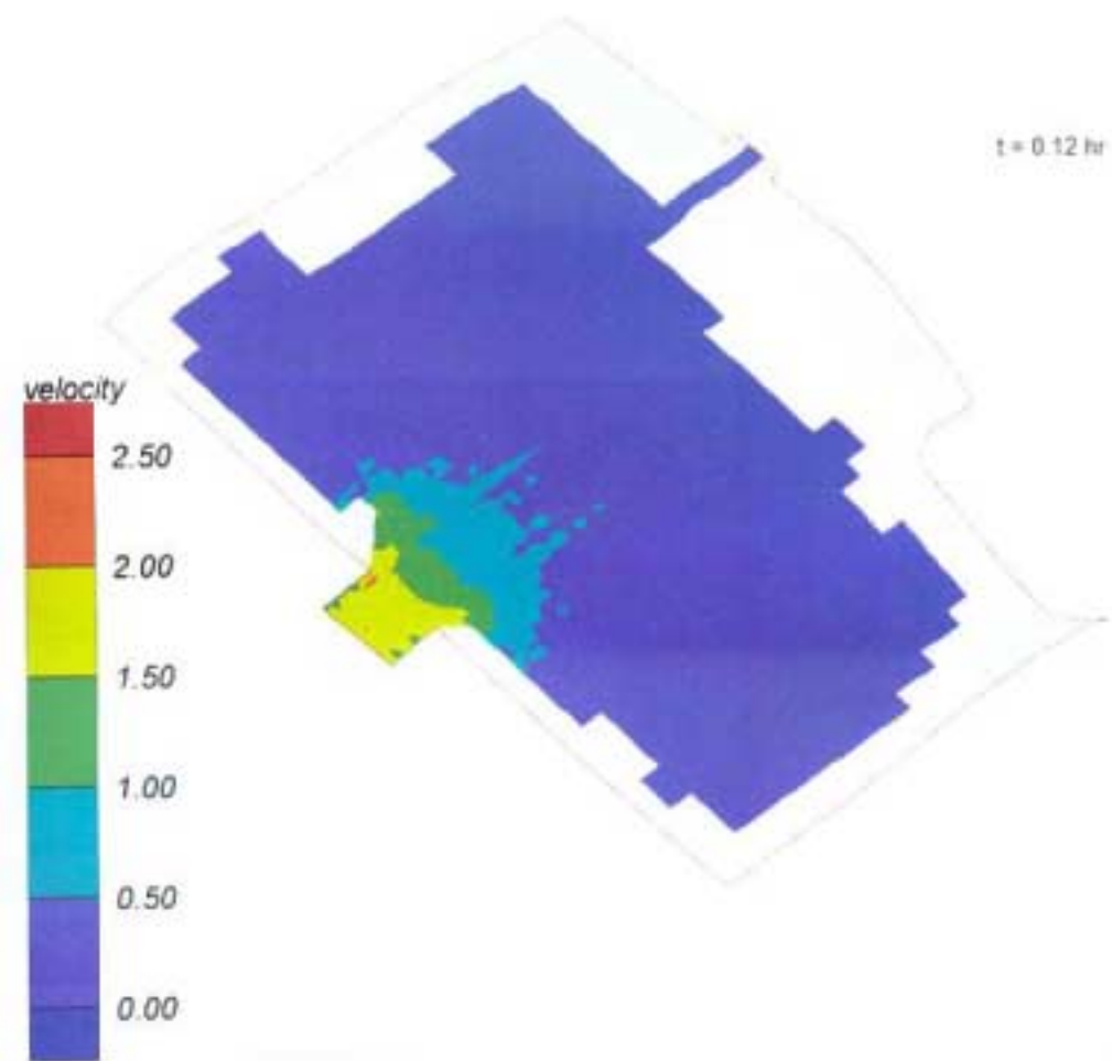
Figure 6.12 Reservoir B Dambreak - Velocity Contours (m/s) and Vectors with 'Sunny Day' Inflow Conditions
