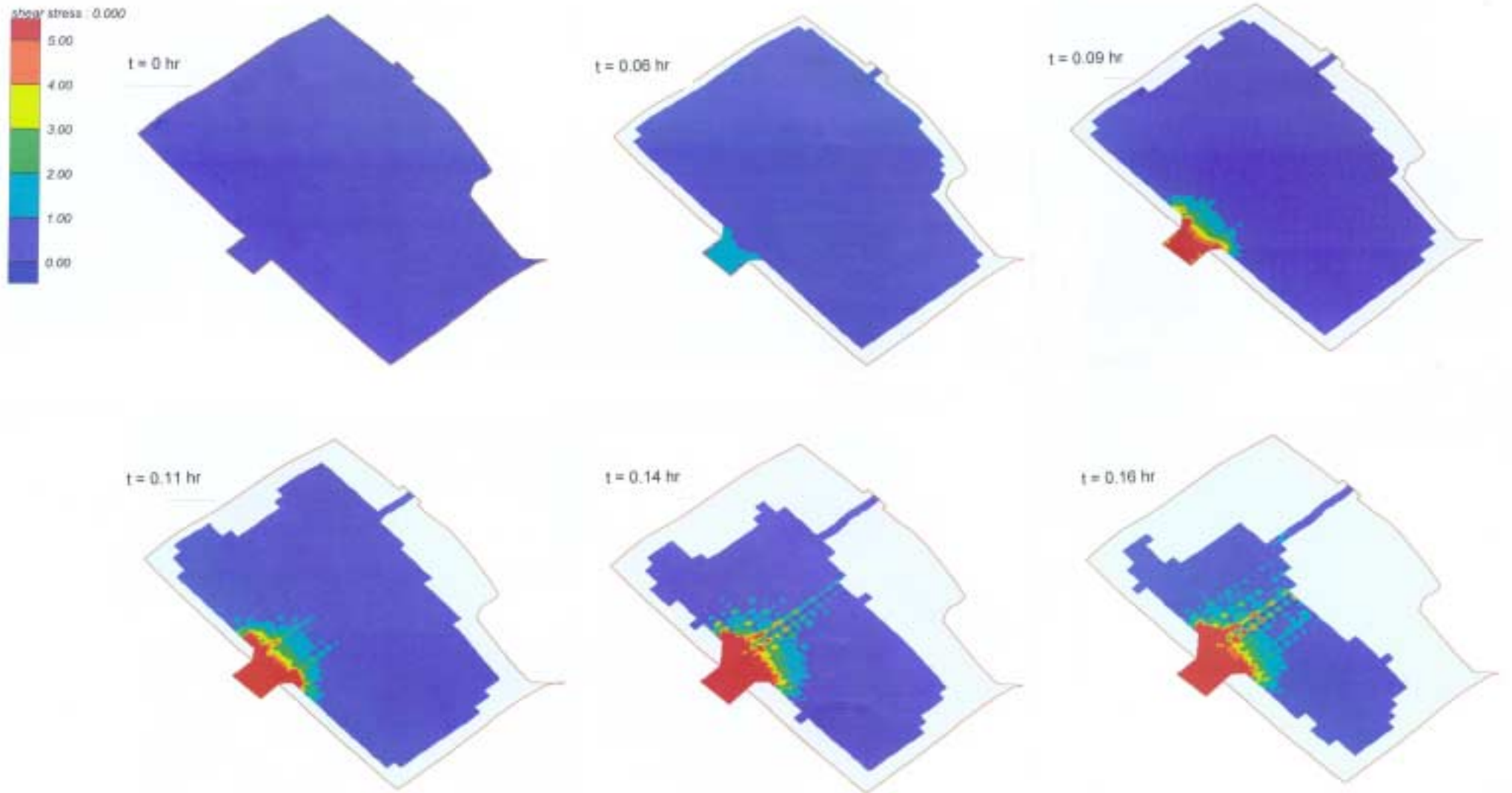
Figure 6.11 Reservoir B Dambreak - Development of Bed Shear Stress (N/m 2 ) with 'Sunny Day' Inflow Conditions
