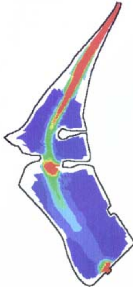
Reservoir A Dambreak – Total erosion depth with 10,000-year Flood Inflow Conditions
