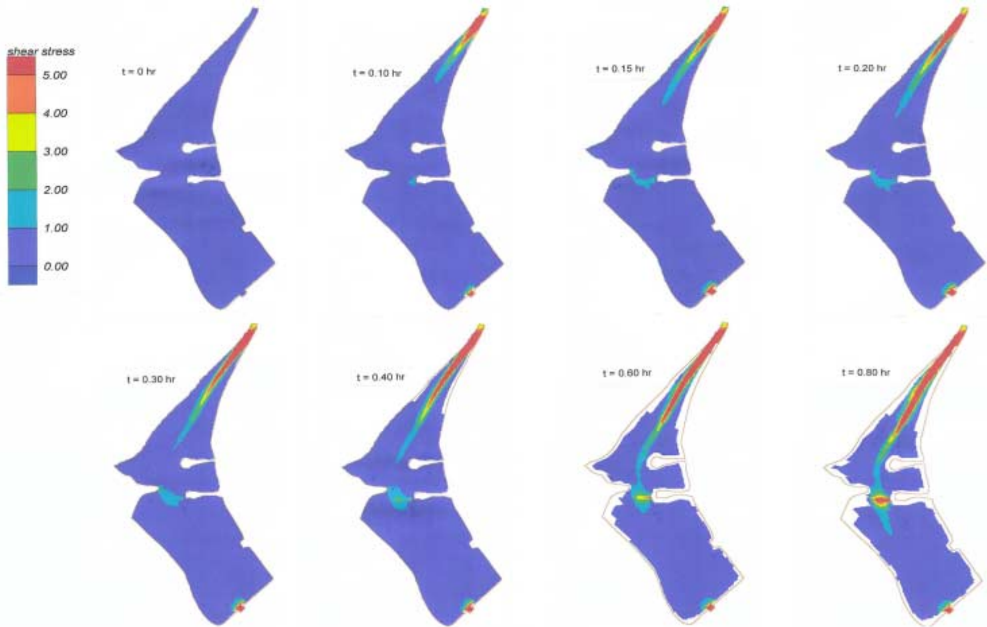
Figure 6.8 Reservoir A Dambreak - Development of Bed Shear Stress (N/m 2 ) with 10,000-year Flood Inflow Conditions
