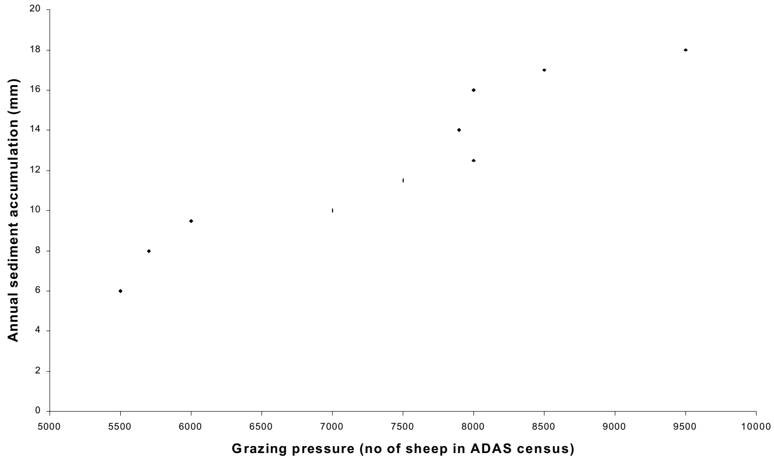
Correlation between annual rate of sediment accumulation in Blelham Tarn and total number of sheep in adjacent parishes (after Van der Post et al , 1997).
