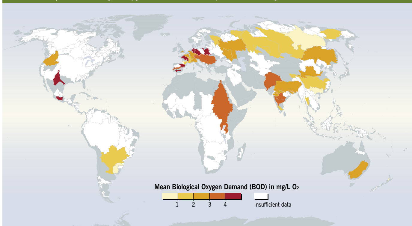
FIGURE 2.14 | Trends in biological oxygen demand (BOD) of major rivers in five regions (1980–2005)
