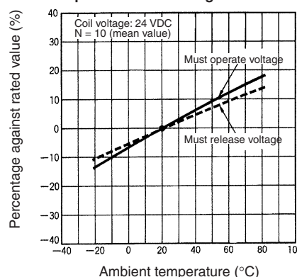
Coil Temperature vs. Must Operate/release Voltage
