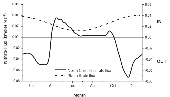
Figure 4. Seasonal fluxes of nitrate N in the Outer Firth of Clyde from marine and riverine sources (from Rippeth and Jones, 1997). Negative flux indicates export of nitrogen form of the Clyde system.
