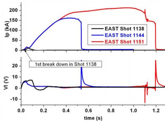
Fig.3 1 st break down and following shots with I_p > 150 kA and 220 kA
