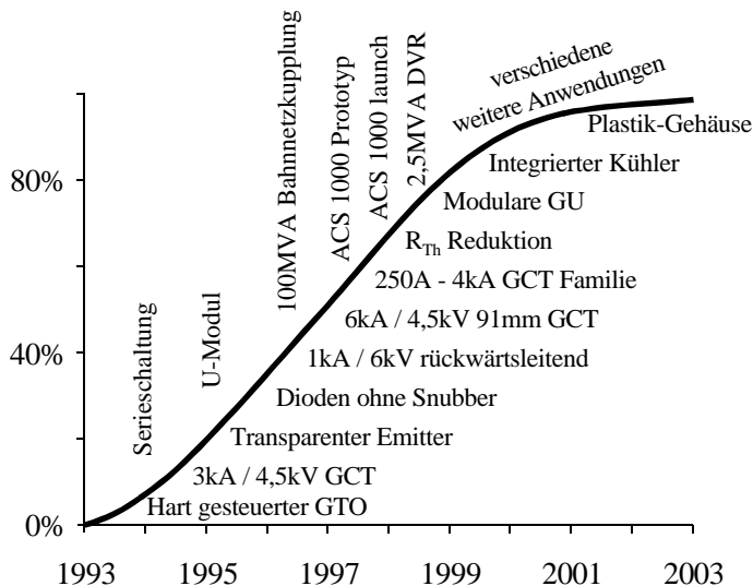
Fig. 12: The development of IGCT components and their application
