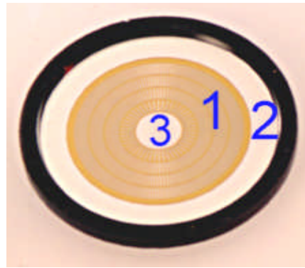
Fig. 5: GCT (1) and diode (2) on the same wafer. The gate has its contact at the centre (3) on the 51 mm disc (6 kV, 520 A).
