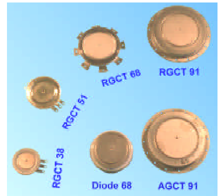
Fig. 7: Reverse conducting GCT with wafer diameters of 38 mm, 51 mm, 68 mm and 91mm and a 91 mm GCT
