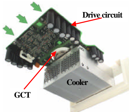
Fig. 6: GCT and drive circuit slide onto the cooler to form a single unit both electrically and mechanically.
