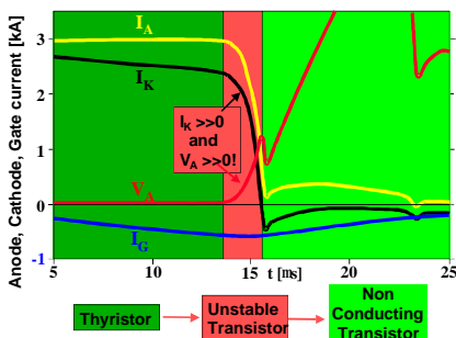
Fig.1: Typical turn-off characteristic of a 4.5kV 3kA GTO.
