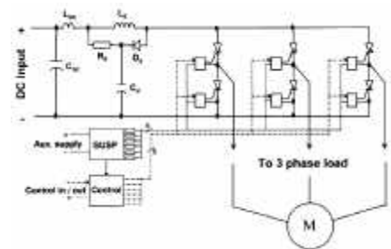
Fig.8: Typical circuit of a three phase IGCT converter. A common supervision unit continually checks switch.
