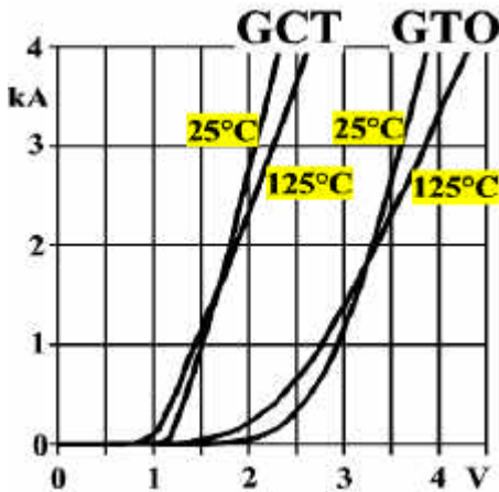
Fig. 4: A comparison between GTO 5SGA 40L4501 and GCT 5SGY 35L4502. The commutation losses of both devices are approximately the same.
