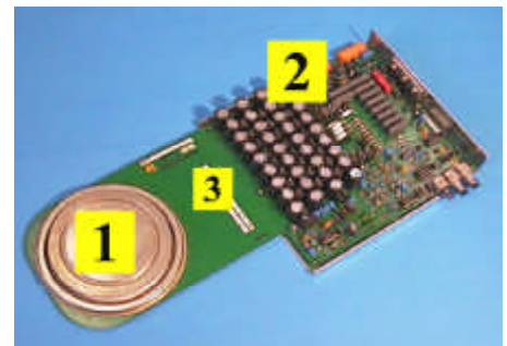
Fig. 3: 4.5kV, 3kA, IGCT (Integrated Gate Commutated Thyristor). The GCT and the gate unit form a single part. The PCB (3) connects the GCT and the drive.
