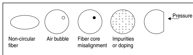
Figure 6. Fiber irregularities
