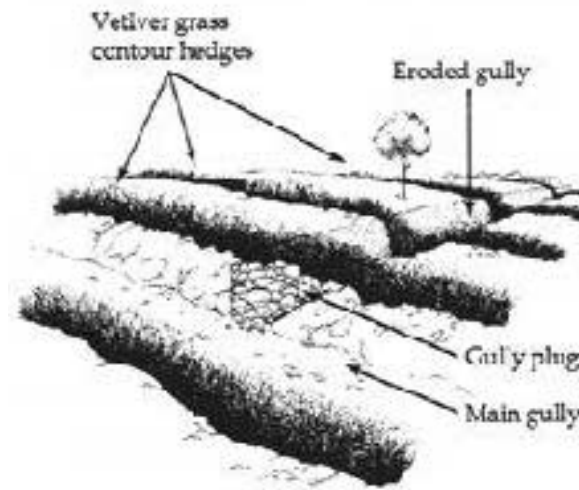
Figure 43. Stabilizing Gullies
