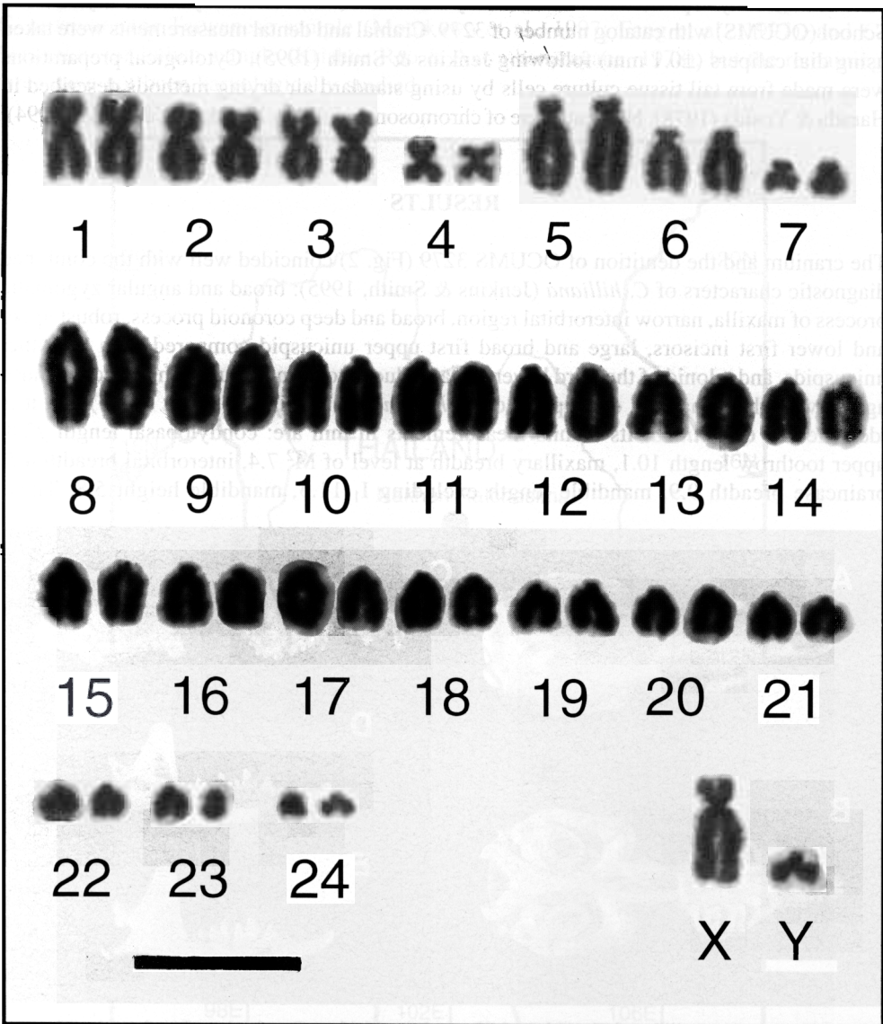
Fig. 3. Conventional karyotype of Crocidura hilliana from Nakhon Ratchasima Province in Thailand (OCUMS 3279). The bar represents 10 \mu m.
