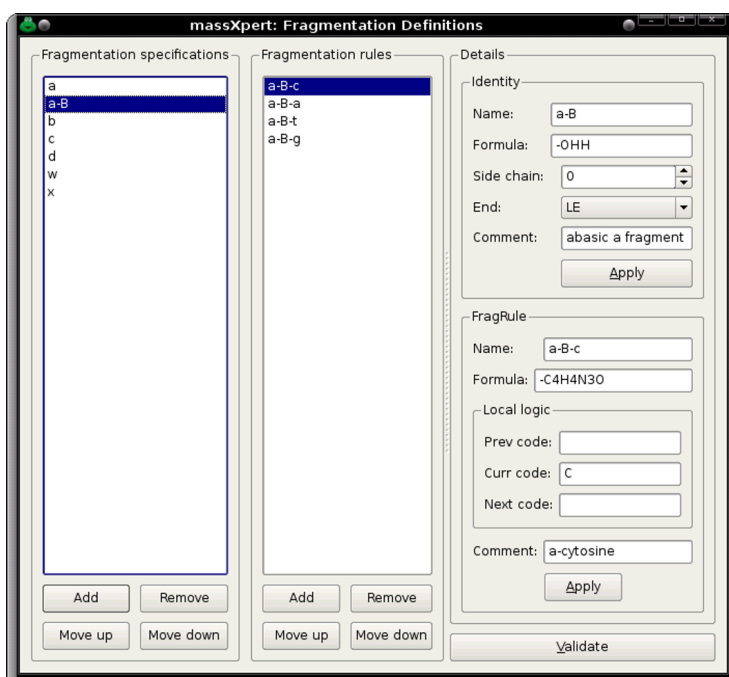
Figure 6.11: XpertDef fragmentation rules definition. Each fragmentation rule is defined using a name, a formula and a local logic, that is a set of logical conditions which must be verified for the fragmentation rule to be applied to the fragment.
