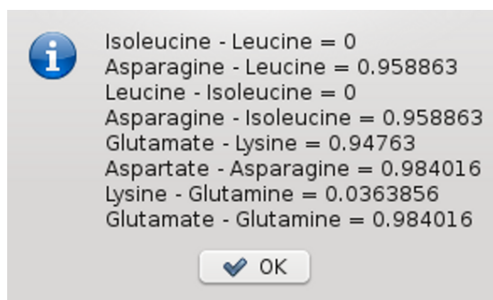
Figure 6.5: XpertDef monomer mass differences. The mass difference between any two monomers in the definition is computed and displayed only if it is less or equal to a threshold (see Figure ??).
