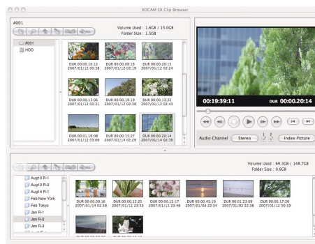
Clip Browser GUI (Macintosh)
