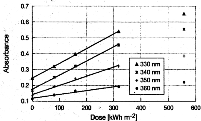
Figure 4 | Change in sample absorbance from Evian® PET bottles exposed to sunlight (test 'EAWAG-2'). Each data point stands for the average of two samples taken from one full and one empty bottle. The lines correspond to linear regressions of the first four data points for each observation wavelength.
