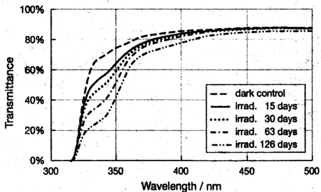
Figure 3 | Transmittance spectra of samples from full Evian® PET bottles exposed to sunlight (test 'EAWAG-2').
