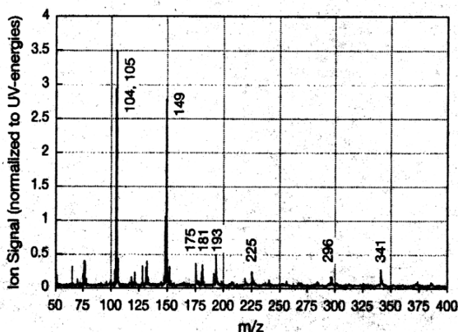
Figure 5 | L2MS mass spectra of PET bottle material (test 'EAWAG-2'). Average of 13 shots on different spots. UV-laser wavelength: 220 nm; UV-laser energies: 5–25 \mu J.
