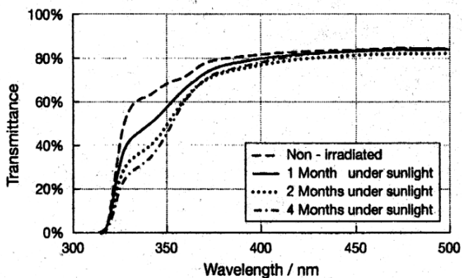
Figure 2 | Transmittance spectra of colourless PET samples exposed to sunlight (test 'EAWAG-1').
