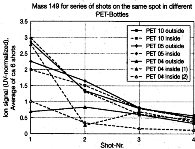
Figure 7 | Depth profiles of the PET fragment at m/z=149 with differently treated PET bottles.
