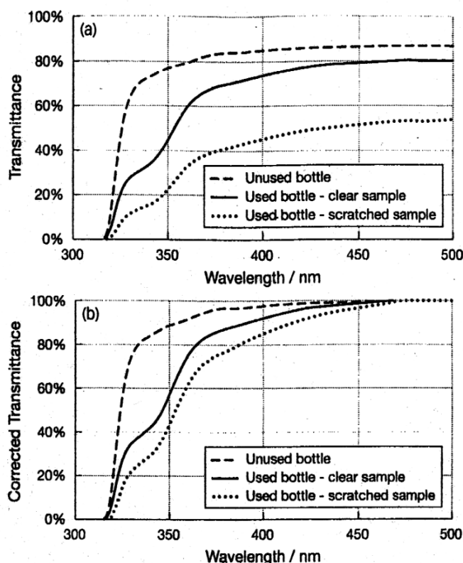
Figure 1 | Uncorrected (a) and corrected (b) transmittance spectra of PET bottles of the same type used in a demonstration project in Thailand. The reduced transmittance of used bottles at visible wavelengths is attributed to scratches on the surface, partly caused by cleaning.
