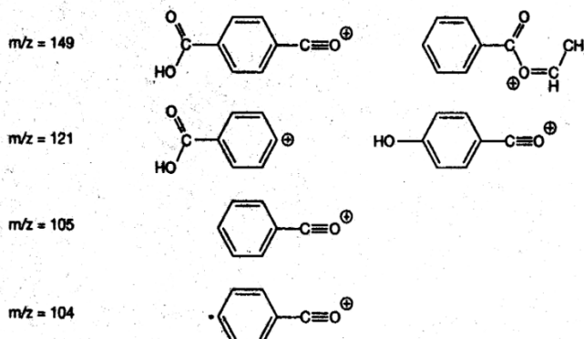
Figure 6 | Rationalised PET fragment masses observed with L2MS.
