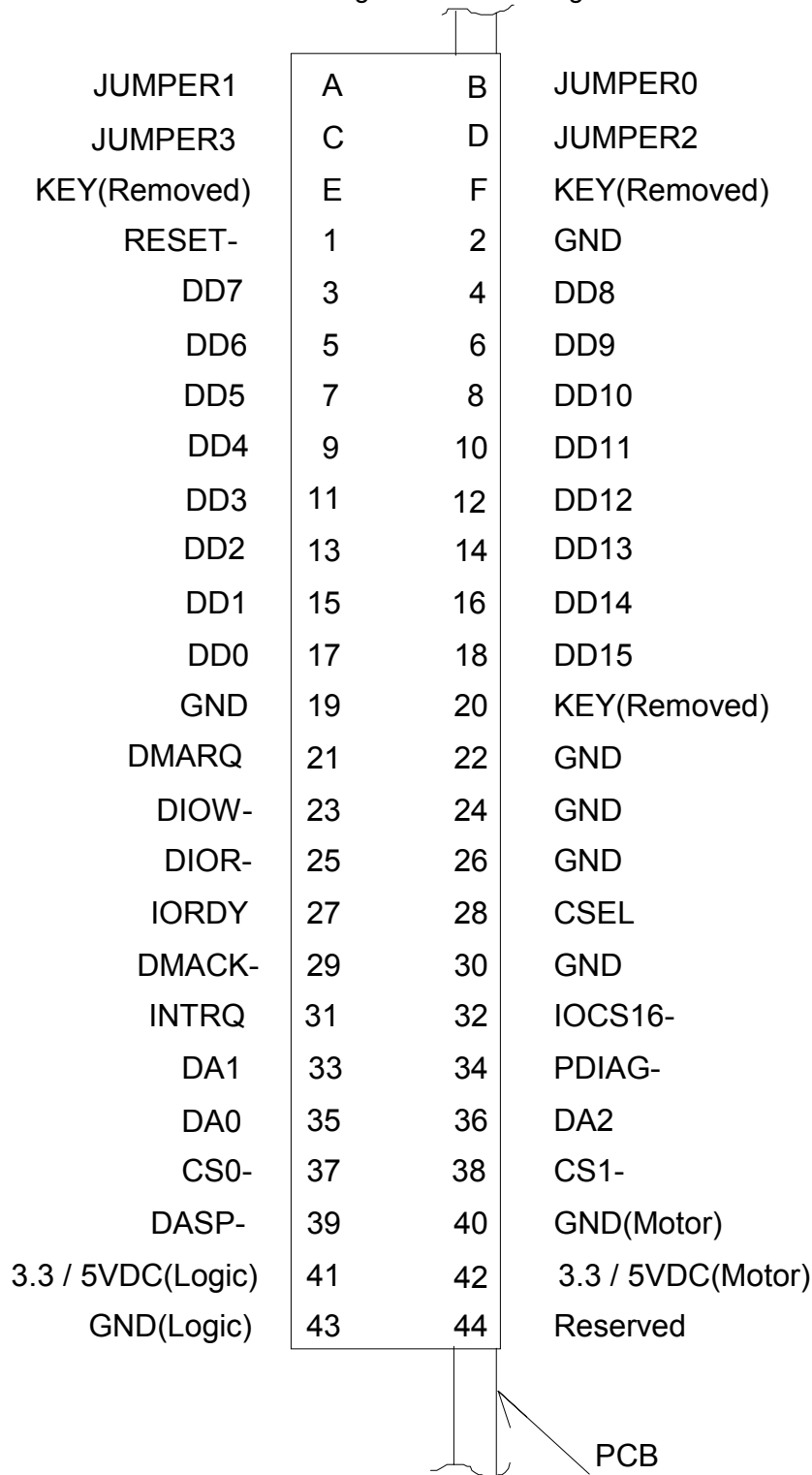
Figure 6-3 Pin Assignments
