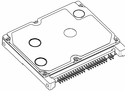
Figure 2-1 Overview of Travelstar C4K40-40 (9.5mm height)
