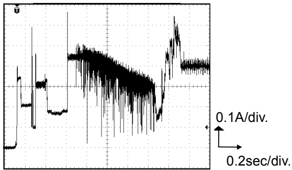
Figure 6-1-1 Power Current Transition (Travelstar C4K40-40)
