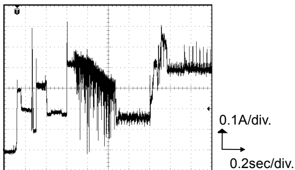
Figure 6-1-2 Power Current Transition (Travelstar C4K40-20)
