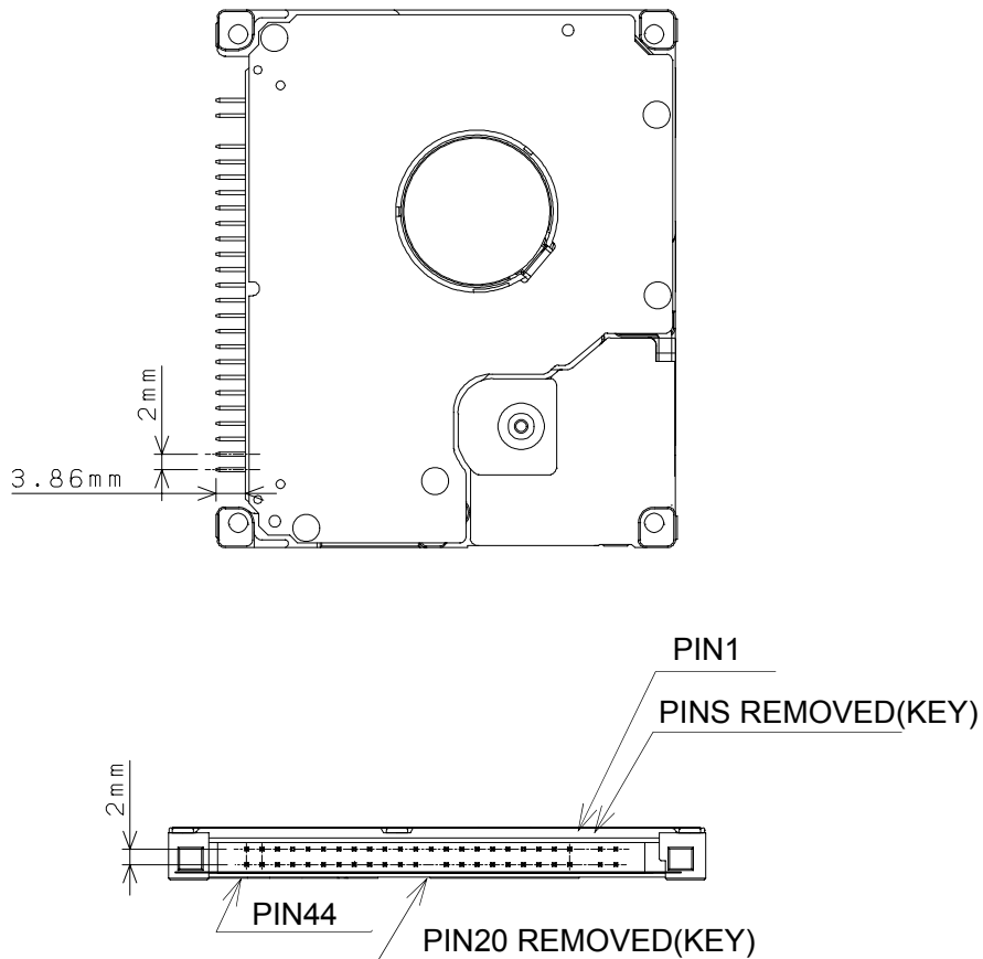
Figure 6-2 Connector Location
