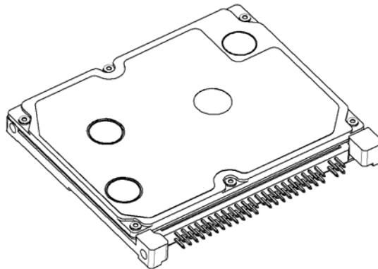
Figure 2-2 Overview of Travelstar C4K40-20 (7.0mm height)
