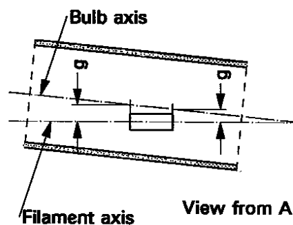
Figure 7 Bulb eccentricity
