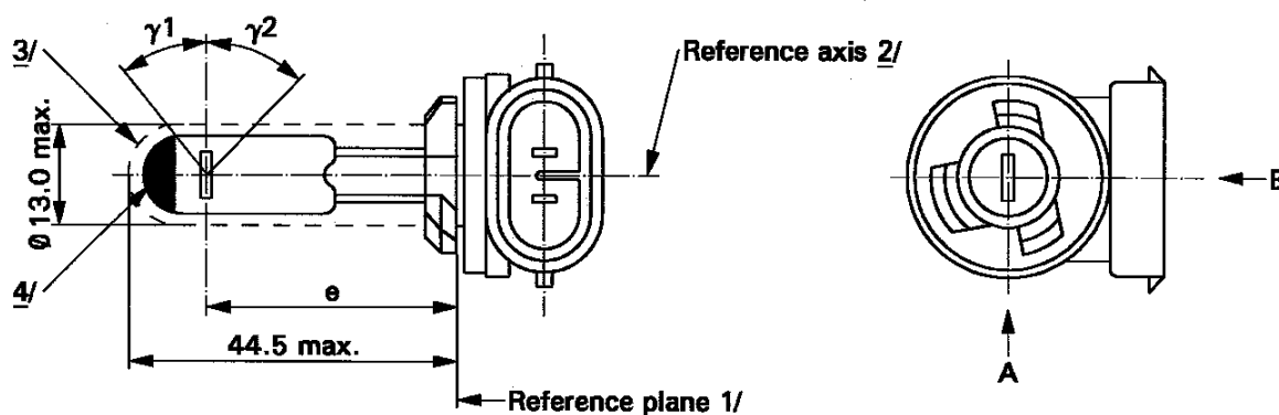
Category H27W/2
