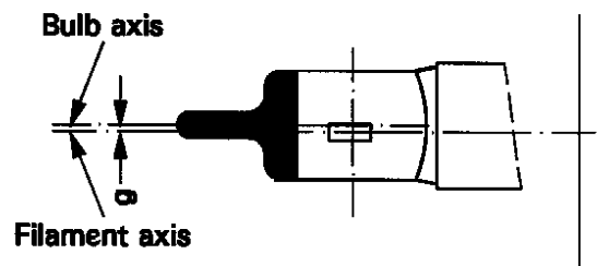
Bulb eccentricity
