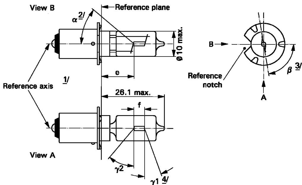
Filament position
