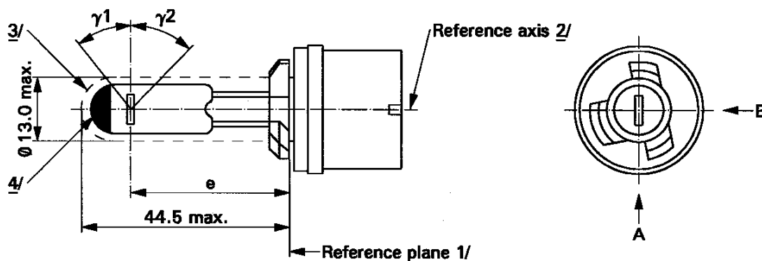
Category H27W/1
