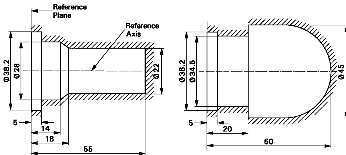
Figure 1 Main drawing
