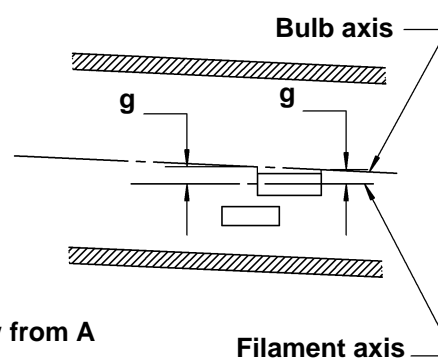
Figure 4 Bulb offset 8/
