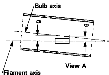
Figure 6 Bulb eccentricity 8/
