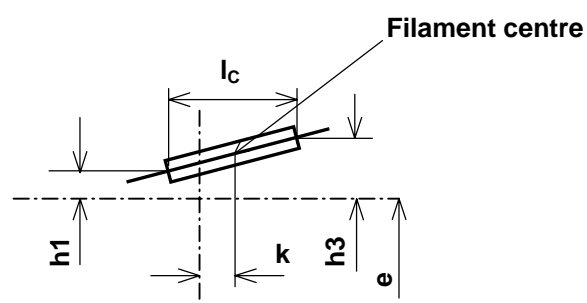
View A of passing-beam filament
