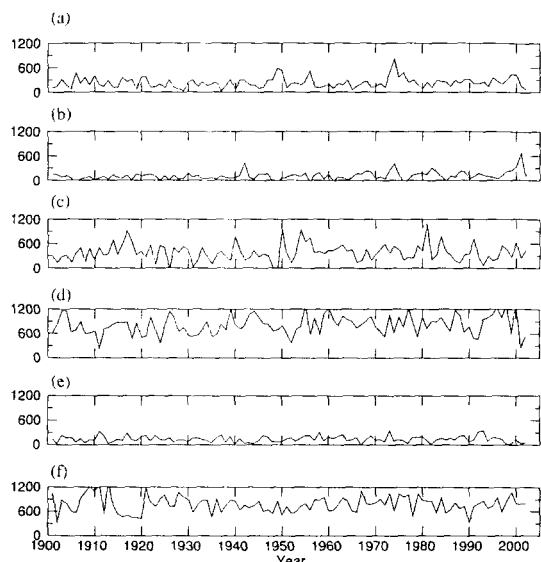
Fig. 7 Australian annual average rainfall teleconnection time series corresponding to the spatial patterns shown in Fig. 6: (a) T1; (b) T2; (c) T3; (d) T4; (e) T5; and (f) T6.
