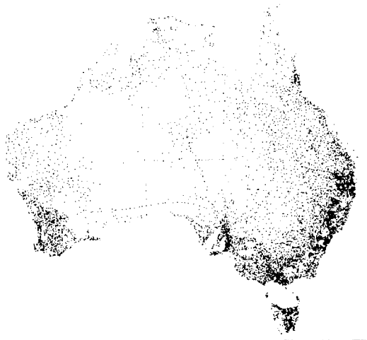
Fig. 1 Location of stations that have reported daily rainfall observations to the Bureau of Meteorology at some time (source: Dean Collins, Bureau of Meteorology).
