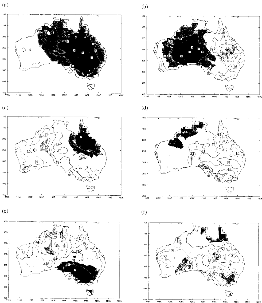
Fig. 6 Australia annual average teleconnection patterns: (a) 'central east' or 'Winton' mode (S1) which explains 60% of the variability in the time series shown in in Fig.1(a); (b) 'central-west' mode (S2) which explains a further 15%; (c) 'north-east' mode (S3) which explains a further 9.5%; (d) 'north-west' mode (S4) which explains a further 3.5%; (e) 'south-east' mode (S5) which explains a further 2.9%; (f) 'Cape York' mode (S6) which explains a further 2.2%.
