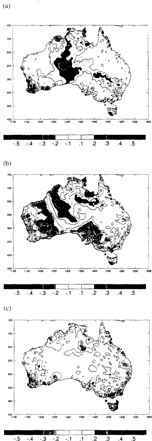
Fig. 4 As for Fig. 3 except for Australian average May to October rainfall.
