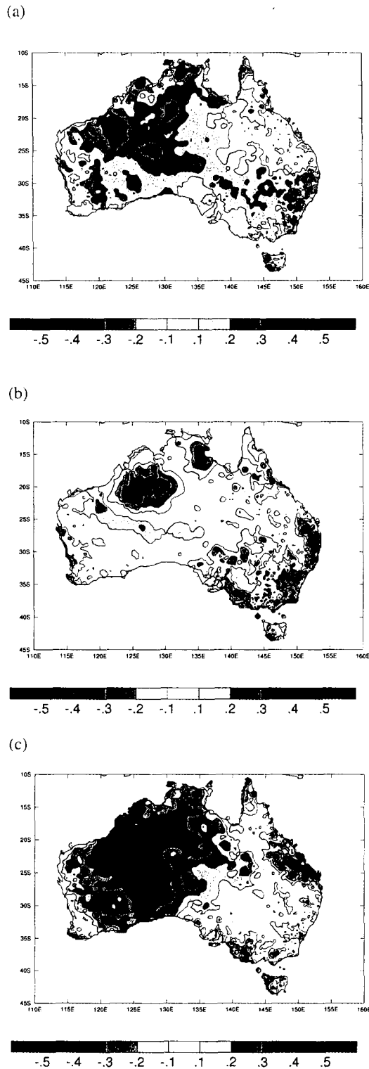
Fig. 5 As for Fig. 3 except for Australian average November to April rainfall .
