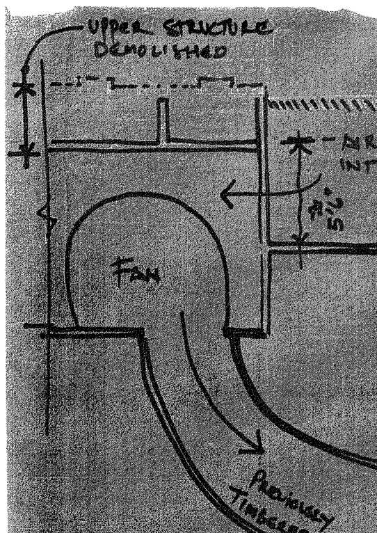
Figure 3. Image taken from Auckland City Council files, photocopy of engineering blueprints, annotated by Bennett following the Princes Street collapse in 2005. Note pocket above blast pad above air shaft
