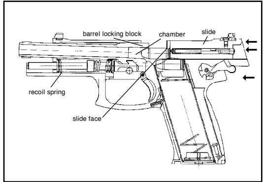
Figure 8 Feeding
