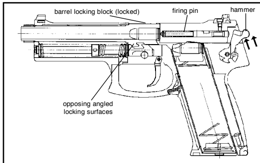
Figure 5 Firing
