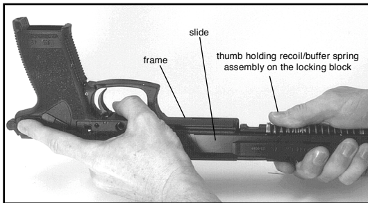
Figure 13 Correct Position for Holding Slide for Reassembly
