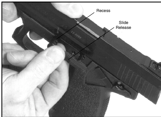
Figure 10 Removing or Installing the Slide Release
