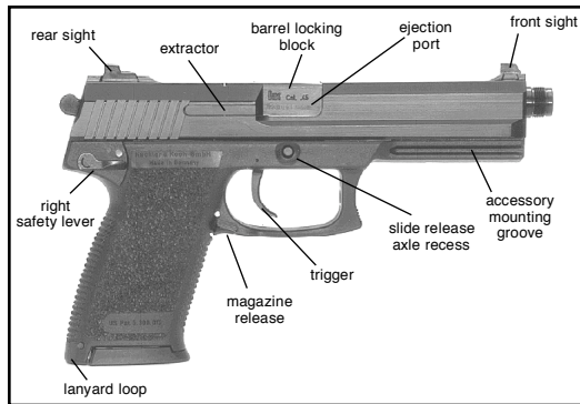
Figure 2 Right View
