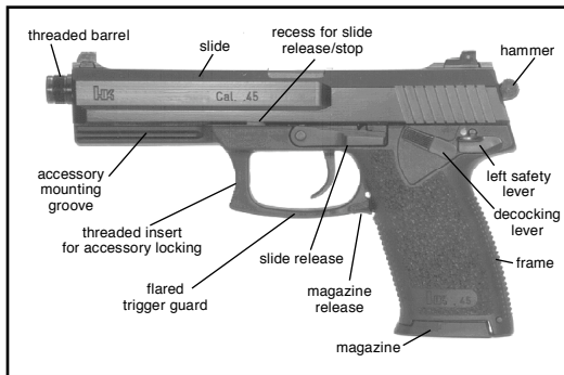
Figure 1 Left View
