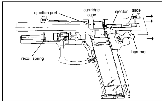
Figure 7 Ejection
