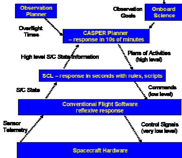
Figure 2. Autonomy Software Architecture
