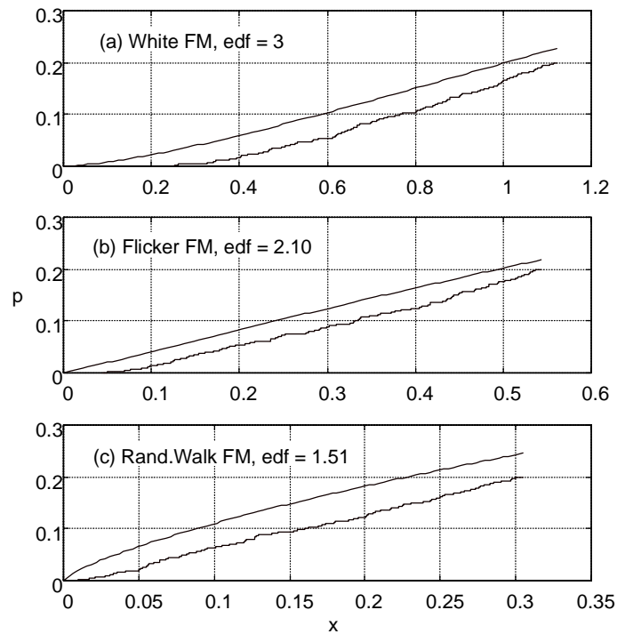
Figure 2. Expanded views of the lower tails of empirical Totvar distribution functions (lower curves), and the corresponding chi-square distribution functions (upper curves)
