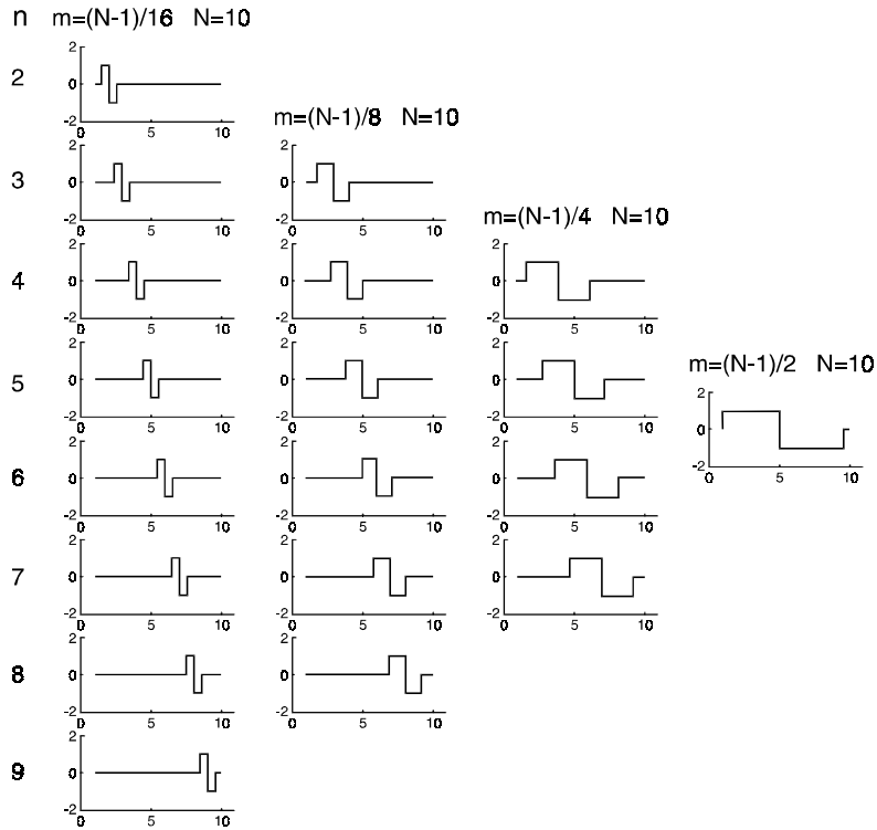
Figure 3. Usual sampling given by Avar for values of m and n when N_x = 10 , m \leq (N_x - 1)/2
