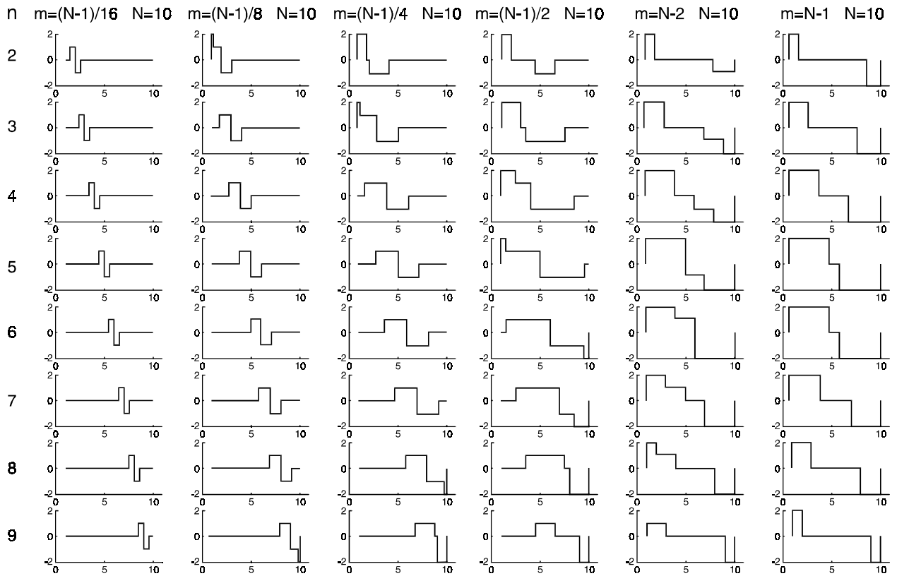
Figure 4. Sampling given by Totvar for values of m and n when N_x = 10 ; note that m is not restricted to m \leq (N_x - 1)/2 as with Avar
