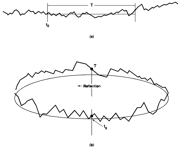
Figure 1. (a) Extension of a phase record by reflection at both ends; (b) circular representation of extended phase record
