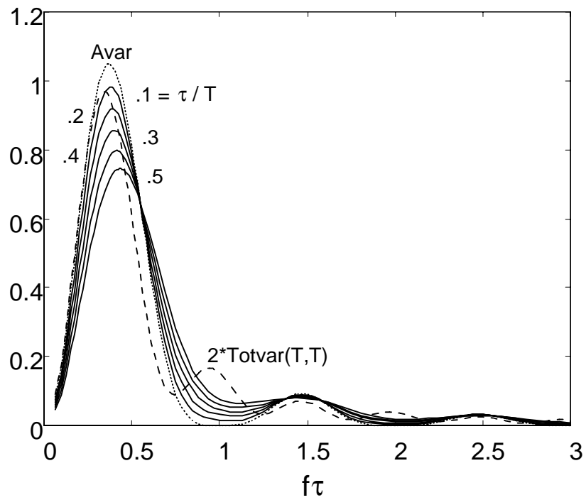
Figure 5. Mean frequency responses of Avar and Totvar as operations on y(t)
