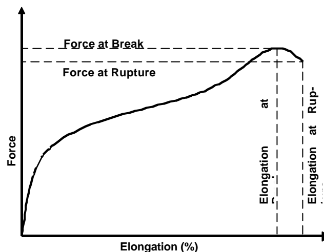
Figure 3.1 : Force-Elongation-Diagram
