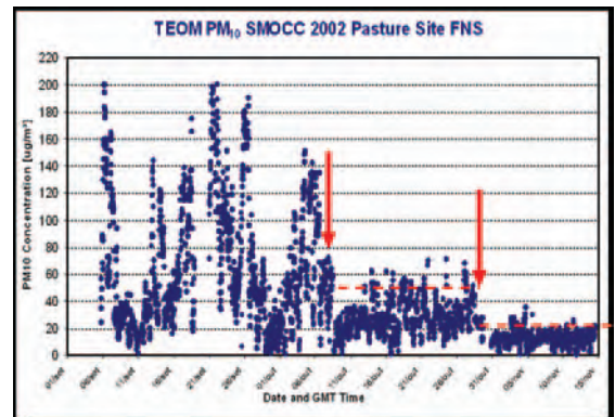
LBA Shows Impact of Aerosols on Clouds (arrows show onset of significant precipitation)
