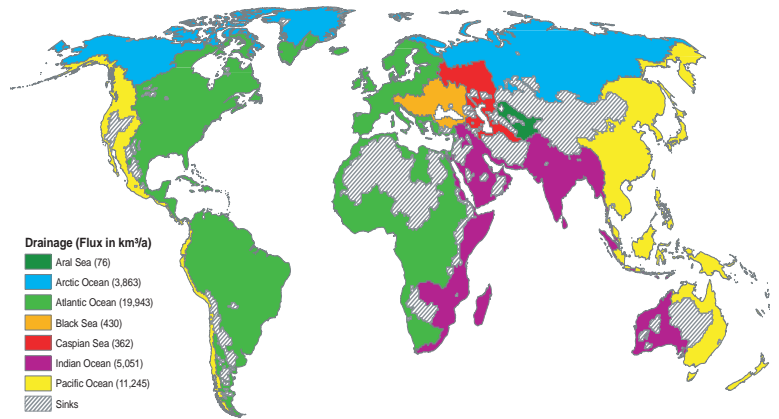
Drainage basins of oceans and seas and associated aggregations of GRDC estimated long term mean annual freshwater influx from rivers.
