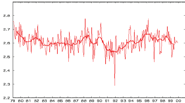
Globally Averaged Precipitation (90N-90S) TOTAL
