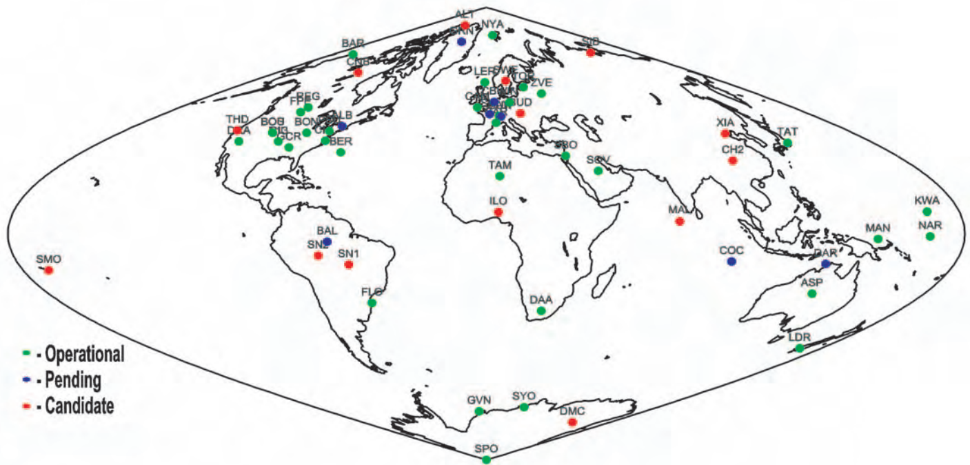
BSRN Station Status, 2004
