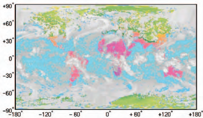
ISCCP Global Cloud Distribution
