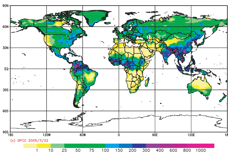
GPCC Monitoring Product Gauge-Based Analysis 1.0 degree precipitation for July 2004 in mm/month
