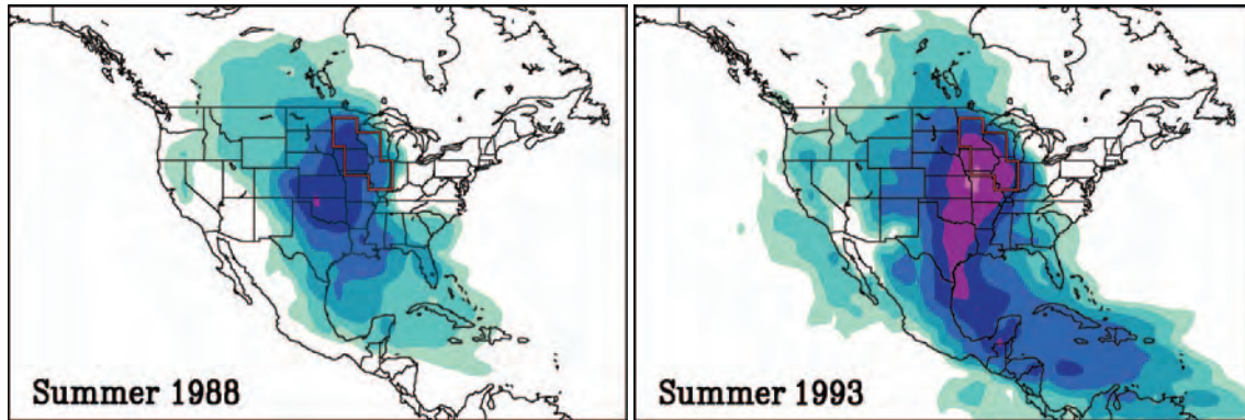
Upstream soil moisture and five-fold increase in Gulf of Mexico moisture flow fuels 1993 flooding.
