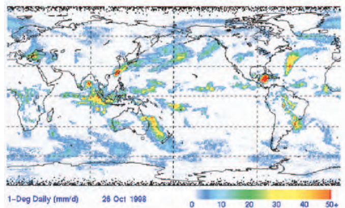
Annual and Daily Global Precipitation from the Global Precipitation Climatology Project (GPCP)
