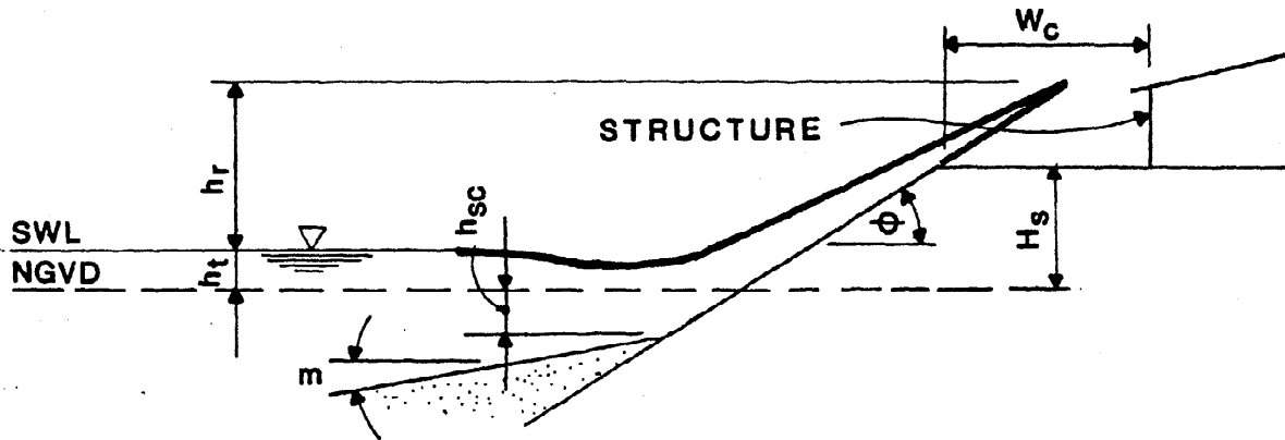
B — PROTECTIVE DEVICE IS ROUGH SLOPE (REVETMENT)
