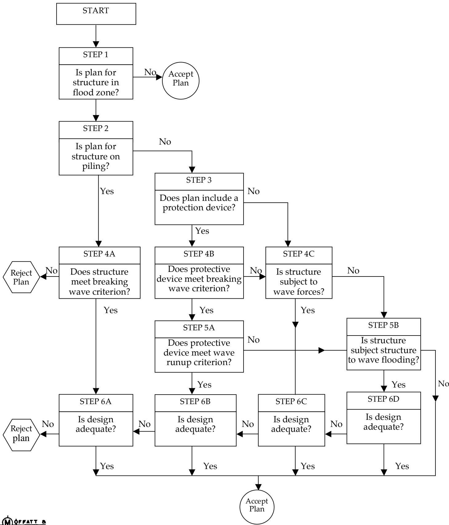
FIGURE 10 PLAN CHECK FLOW DIAGRAM
