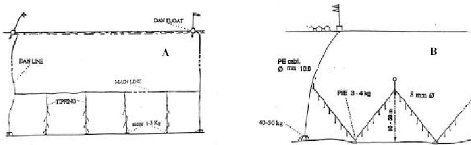
Fig 11: Longline gear directed at deep water sharks and deep-water teleosts during exploratory fishing on the Galicia Bank (EC FAIR, 1999).
