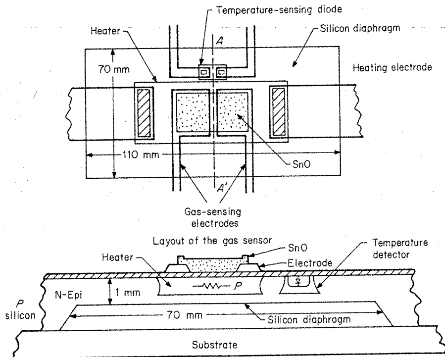
Fig. 26-51. Structure of a silicon substrate gas sensor.
