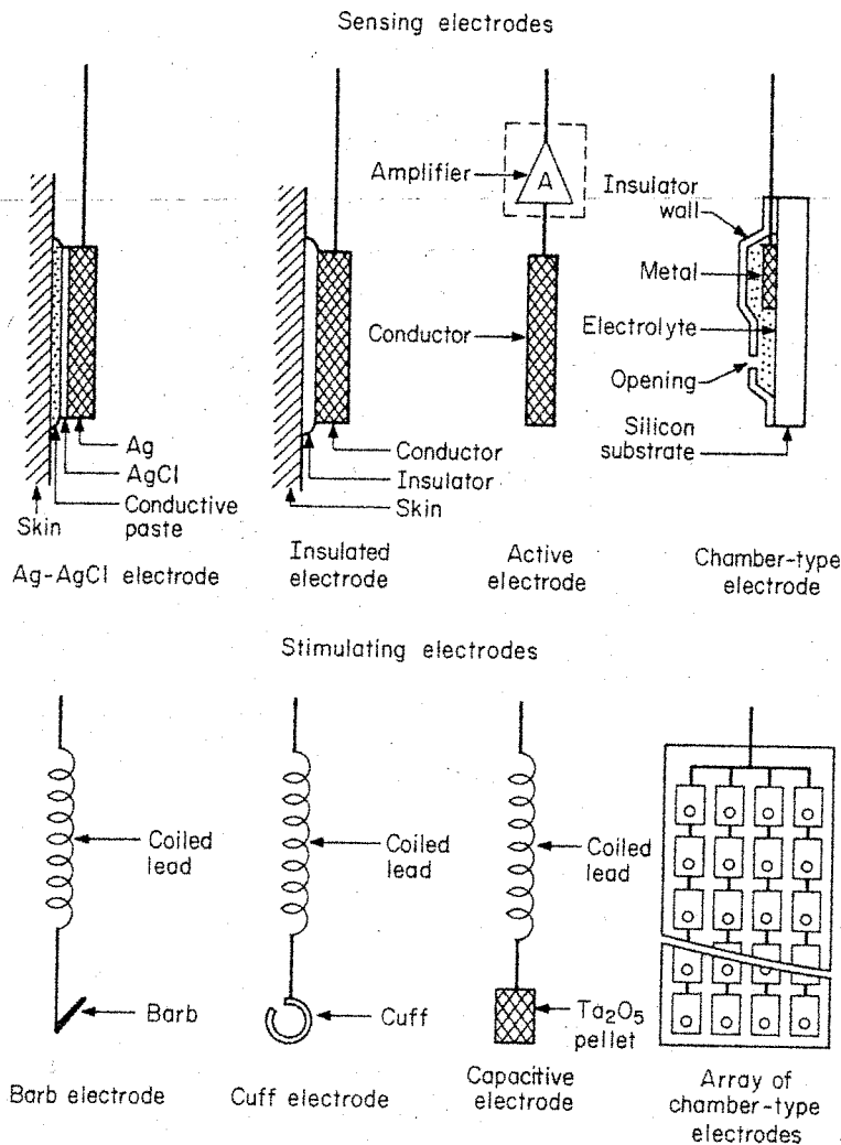
Fig. 26-46. Types of electrodes.
