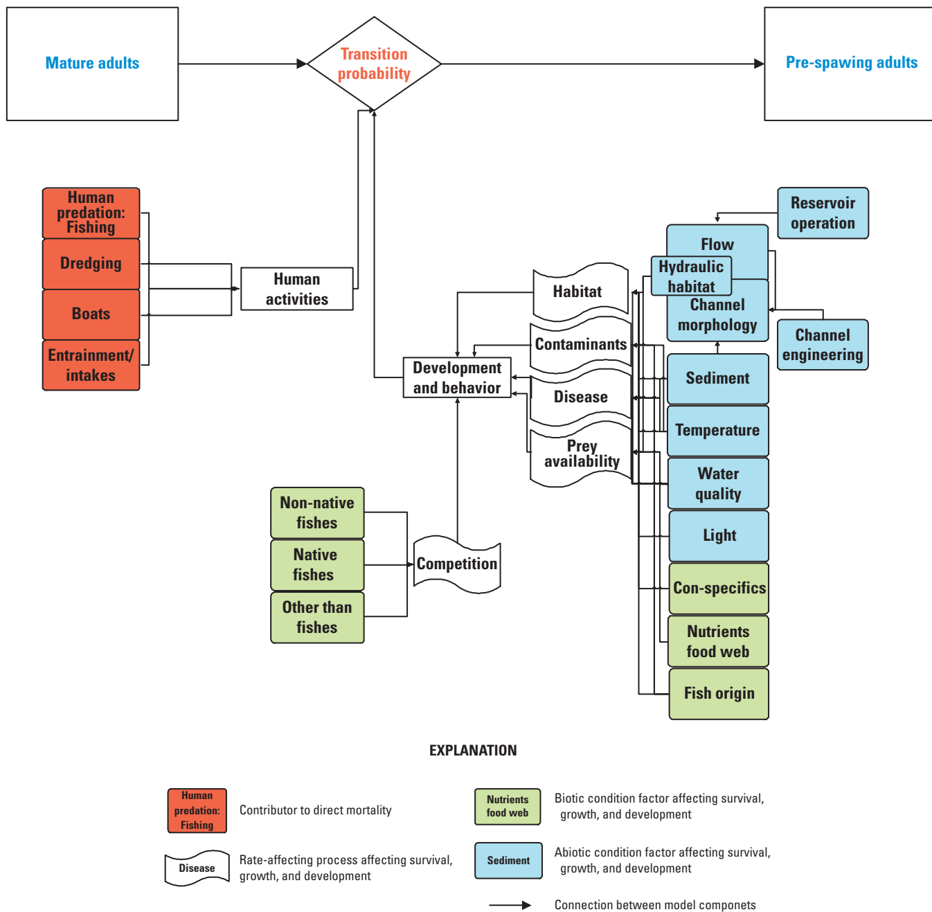
Figure 4. Submodel for the transition from mature to pre-spawning adult in the Scaphirhynchus sturgeon life-history conceptual model.
