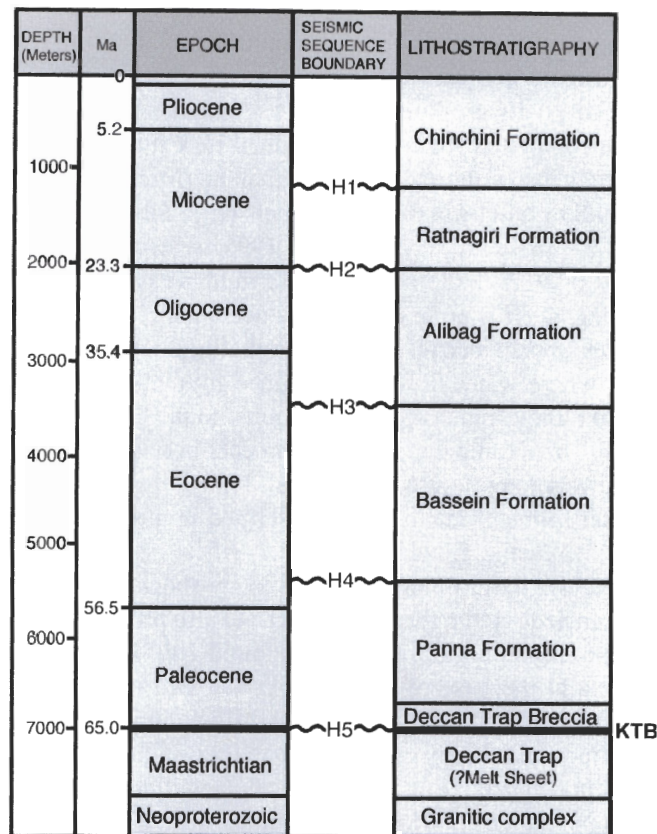
Figure 5. Generalized stratigraphy of the Shiva crater (modified from Basu et al. 1982; Bhandari and Jain 1984; Mathur and Nair 1993; Rao and Talukdar 1980; Wandrey 2004; Zutshi et al. 1993). The oldest sedimentary units in the crater basin, the Deccan Trap breccia, the early Paleocene Panna Formation, and the Deccan Trap floor, bracket the age of the crater at the KT boundary time.
