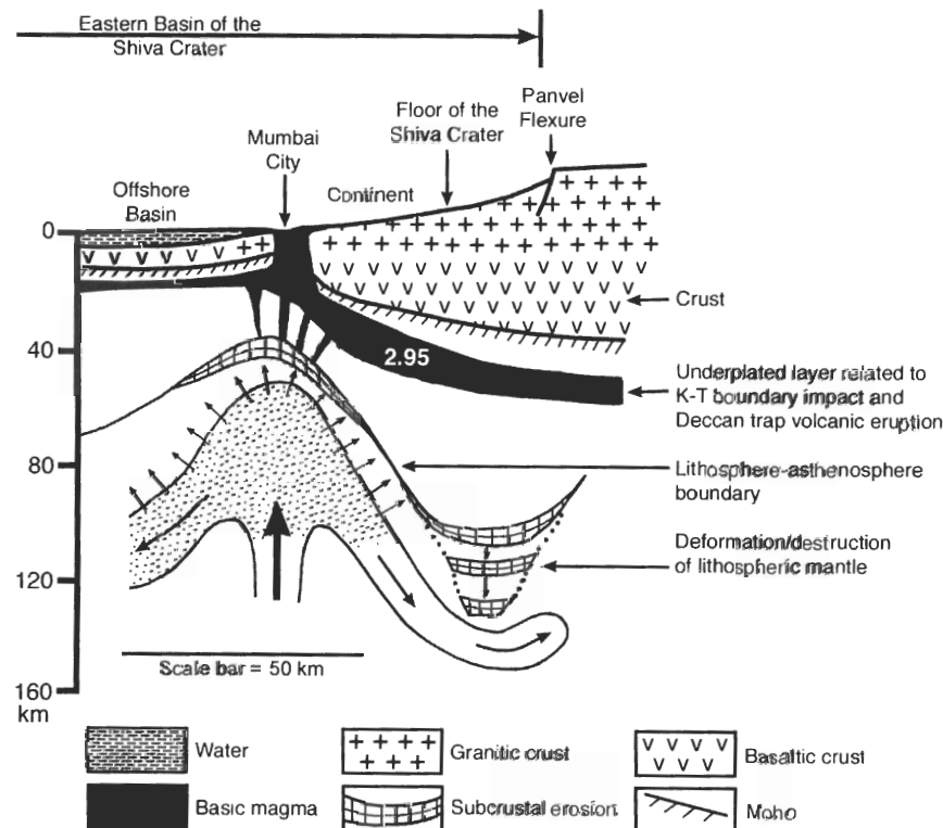
Figure 9. Schematic diagram of the eastern part of the Shiva crater near Mumbai coast to show the upwarping of the mantle more than 50 km and the possible deformation and destruction of the lithosphere because of Shiva impact; on the right side of the drawing, east of Mumbai, thick Deccan lava pile was removed to show the floor of the Shiva crater (modified from Kaila et al. 1981; Pandey and Agarwal 2001).
