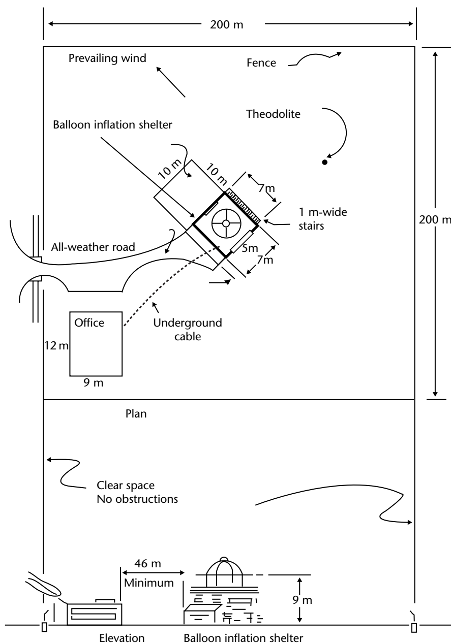
Figure III.11. Upper-air site
