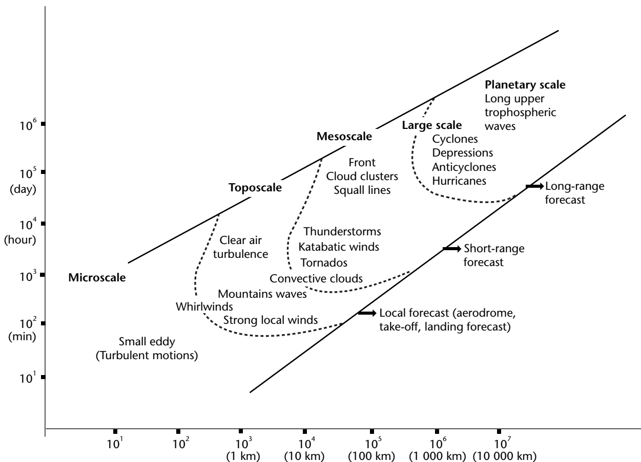
Figure II.1. Horizontal scales and timescales of meteorological phenomena
