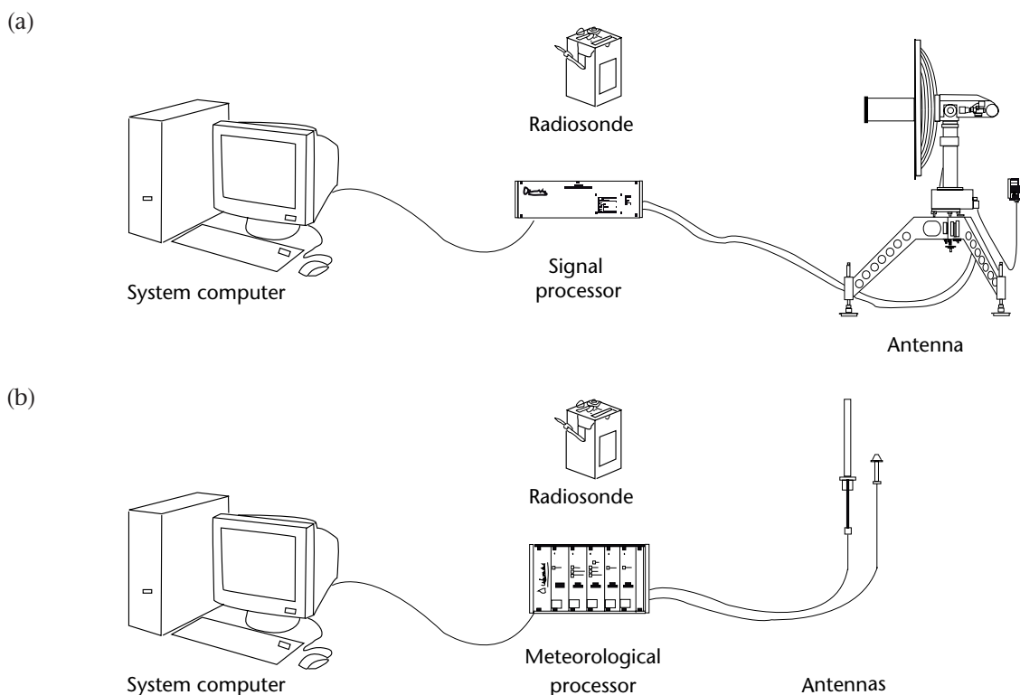
Figure III.14. RDF (a) and GPS (b) upper-air sounding systems
