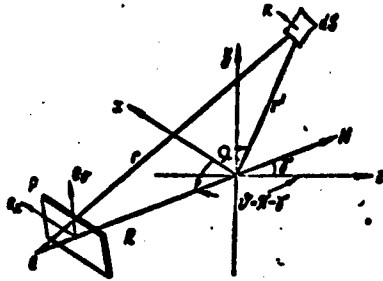
Figure 69. The problem of electromagnetic wave diffraction by an arbitrary metal body.
