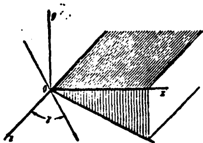
Figure 14. Diffraction by a wedge with oblique incidence of a plane wave. \gamma is the angle between the normal to the incident wave front and the z axis.
