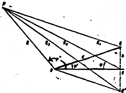
Figure 46. Diffraction of a cylindrical wave by a half-plane. The functions u introduced here Q is the source, Q^* is the mirror image of the source, and P is the observation point. 0 < \varphi'' < \pi are determined (for the values 0 < \varphi' < \pi ) by the equations
