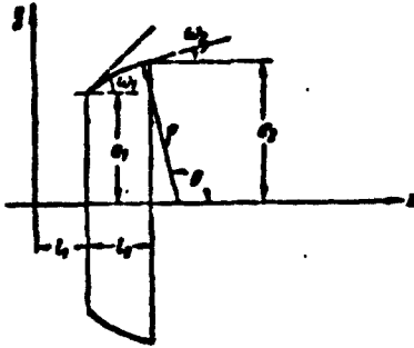
Figure 41. A ring cut from the surface of its sphere by the planes z = l_1 and z = l_1 + l_2 .
