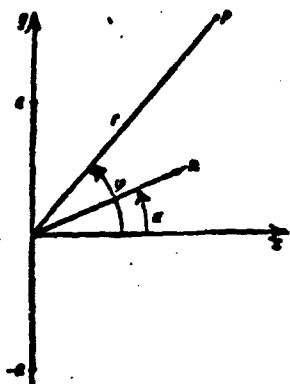
Figure 45. The transverse cross section of a strip with the plane xoy , x = 0 , y = a and x = 0 , y = -a are the coordinates of the strip's edge; n is the normal to the incident plane wave front.
