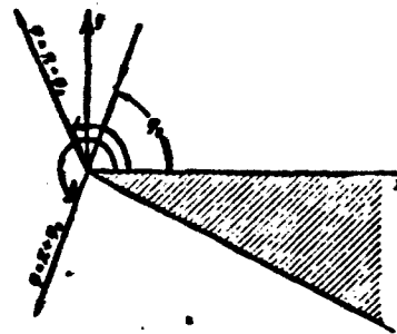
Figure 5. Diffraction of a plane wave by a wedge. The plane wave irradiates only one face of the wedge. \phi_0 is the angle of incidence. The line \phi = \pi - \phi_0 is the boundary of the reflected plane wave, and the line \phi = \pi + \phi_0 is the boundary of the shadow.
