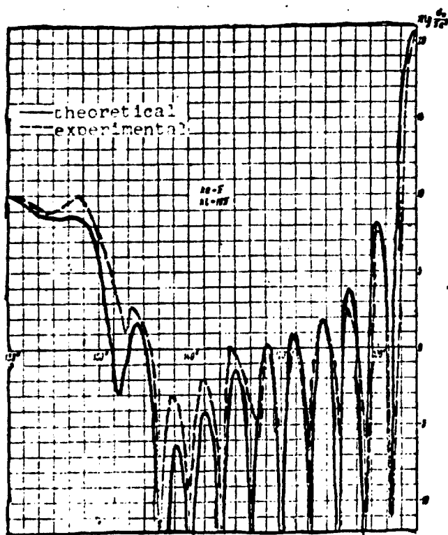
Figure 26. Diagram of the effective scattering surface for a finite cylinder. The case of H-polarization.
