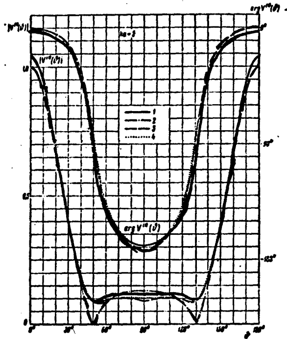
Figure 67. The function V^{(1)}(\theta) for a disk with normal incidence of a plane wave (curve 4). Curves 1, 2 and 3 from Figure 20 are drawn for comparison.
