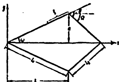
Figure 28. Diffraction of a plane wave by a conical body. The plane wave is propagated along the z axis.
