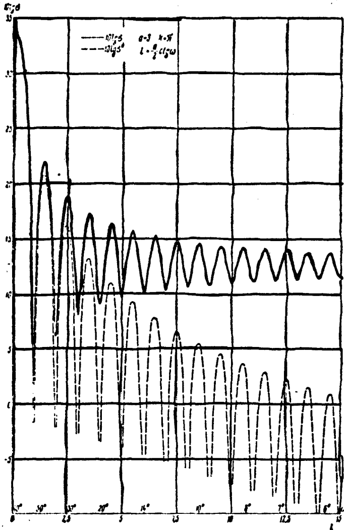
Figure 38. The effective scattering area of a finite paraboloid as a function of its length with a constant radius of the base.
