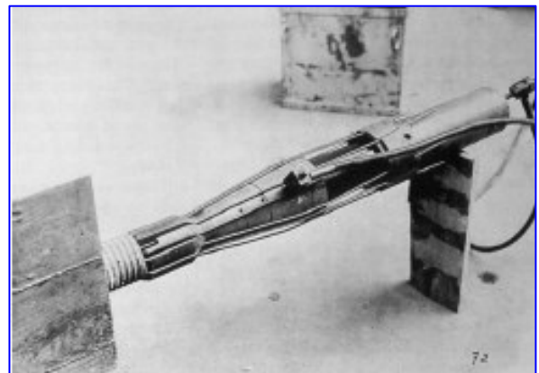
Martinetto Freyssinet
