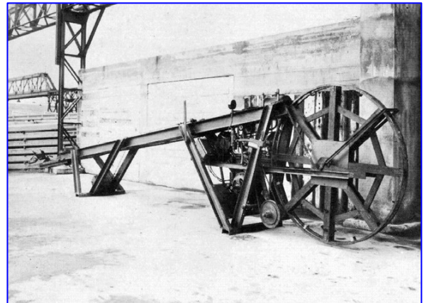
Martinetto Freyssinet
