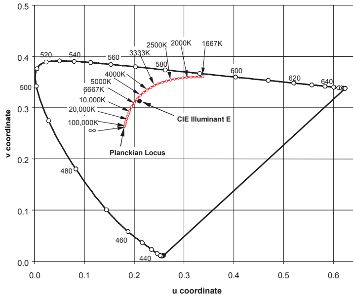
Figure 4. 1960 CIE UCS (u, v) color space.
