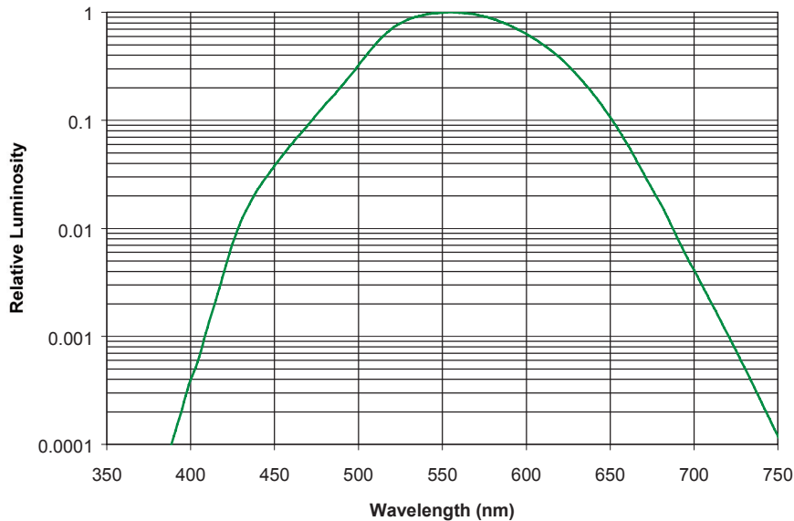
Figure 1. 1931 CIE luminosity function.
