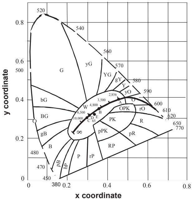
Figure 3. 1931 CIE Color Space.
