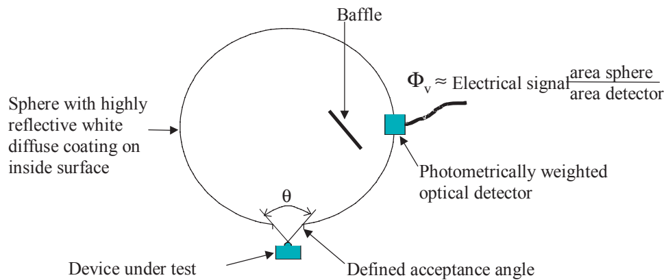
Figure 12. Luminous Flux Test System.
