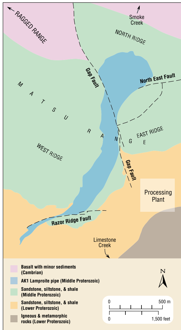
Figure 4. The tadpole-like shape of the Argyle AK1 lamproite pipe, which is broadest to the north and narrowest to the south, is evident in this simplified geologic map. The pipe is located within resistant rocks of the Matsu Range that here form the East and West Ridges.
