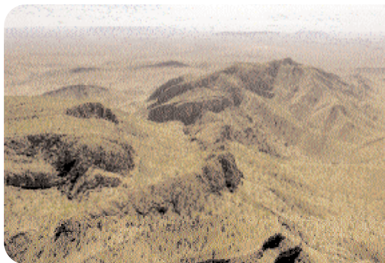
Figure 6. This 1983 aerial photograph (looking northeast) shows the valley in the Matsu Range (slightly to the left of center here) where the Argyle AK1 lamproite pipe was discovered after extensive regional exploration for diamonds. Lake Argyle is visible in the distance. The orientation of this photograph, which was taken before diamond-mining operations began, is opposite that of the photo in figure 1. Today, most of this valley floor is occupied by the Argyle open pit.
