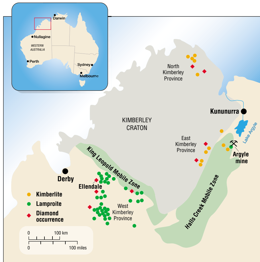
Figure 3. This generalized sketch map shows the locations of kimberlites, lamproites, and diamond occurrences in the Kimberley craton region of Western Australia. The Argyle mine is situated east of the Kimberley craton, near the eastern margin of the Halls Creek Mobile Zone. Other diamond deposits (not yet developed) are located at Ellendale to the southwest of the craton, and at two kimberlites within the northern part of the craton. The first Australian diamonds were found by gold prospectors in alluvial deposits near Nullagine (see inset) in 1895. Adapted from Atkinson et al. (1984b, figure 3B).
